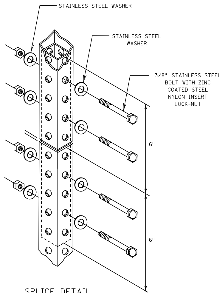
SPLICE DETAIL
