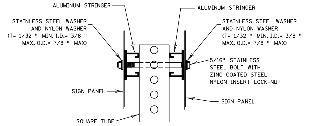
BACK TO BACK SIGN MOUNTING WITH STRINGERS
