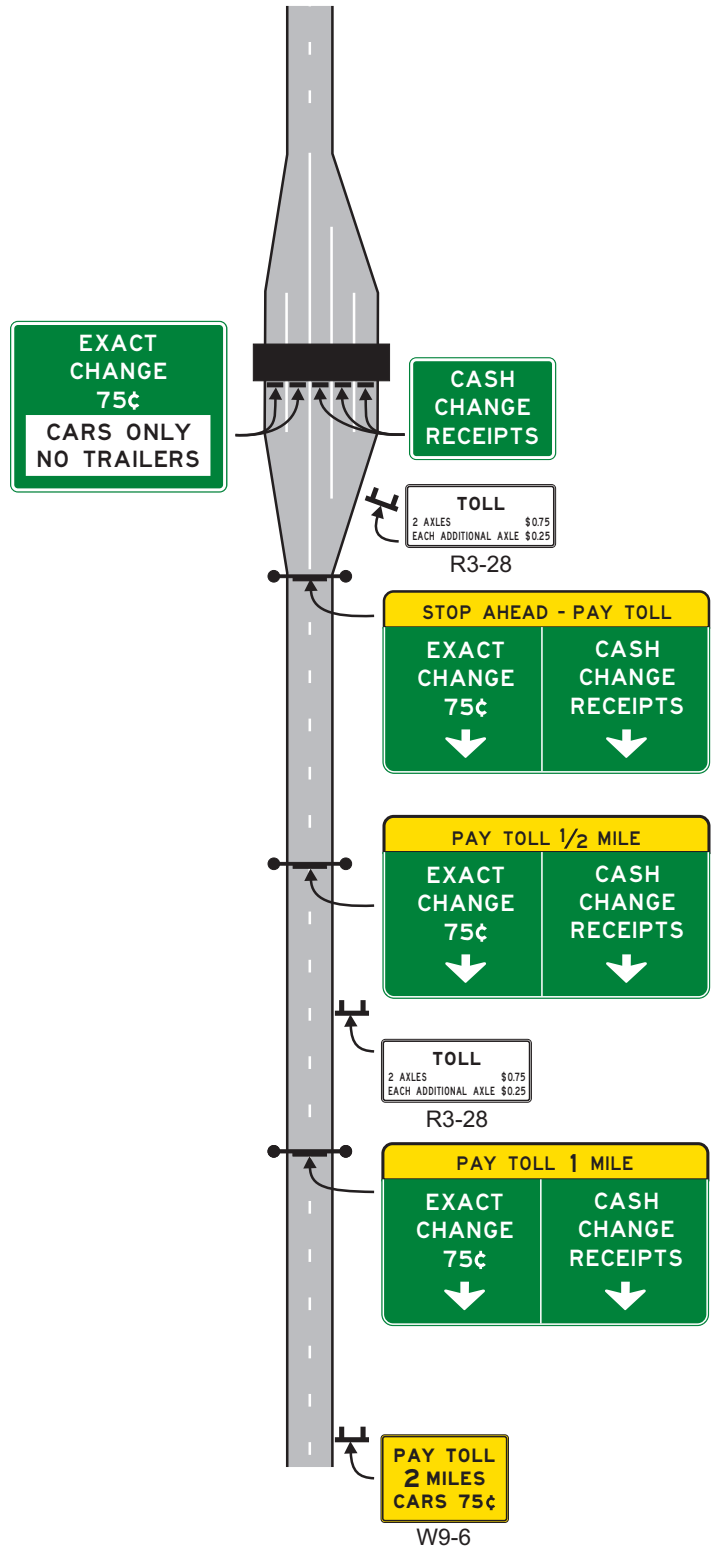
Figure 2F-10 Examples of Mainline Toll Plaza Approach and Canopy Signs
