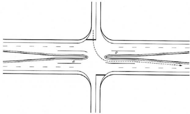
Figure E-10. Left-turn acceleration lanes (from Mn/DOT)
