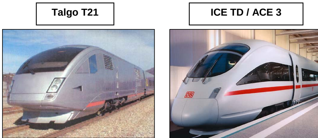
Figure 3.17. “Generic 110-mph Train Options” Represented by Talgo T-21 and Tilting DMU
