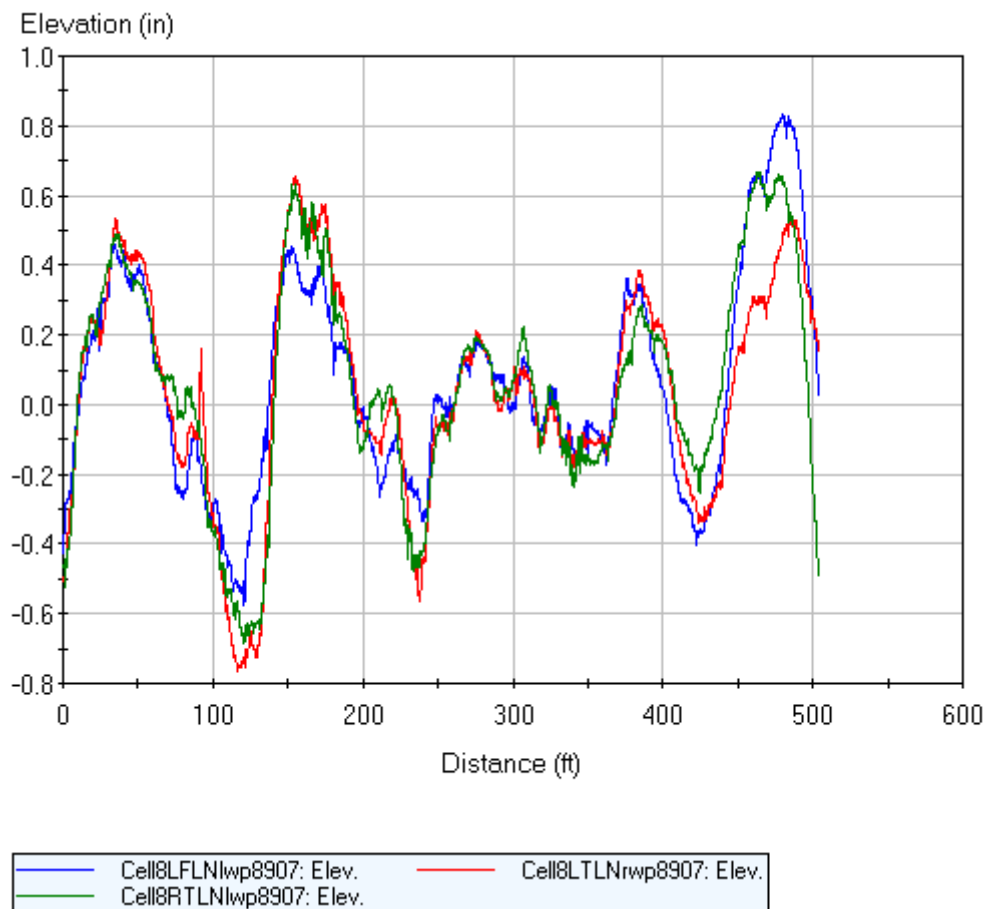
Figure B.3. Cell 8 pre-grind ProVAL report.
