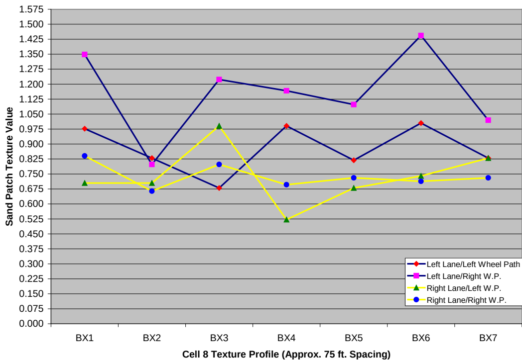
Figure 4.13. Sand volumetric technique ASTM E-965 test result on Cell 8.
