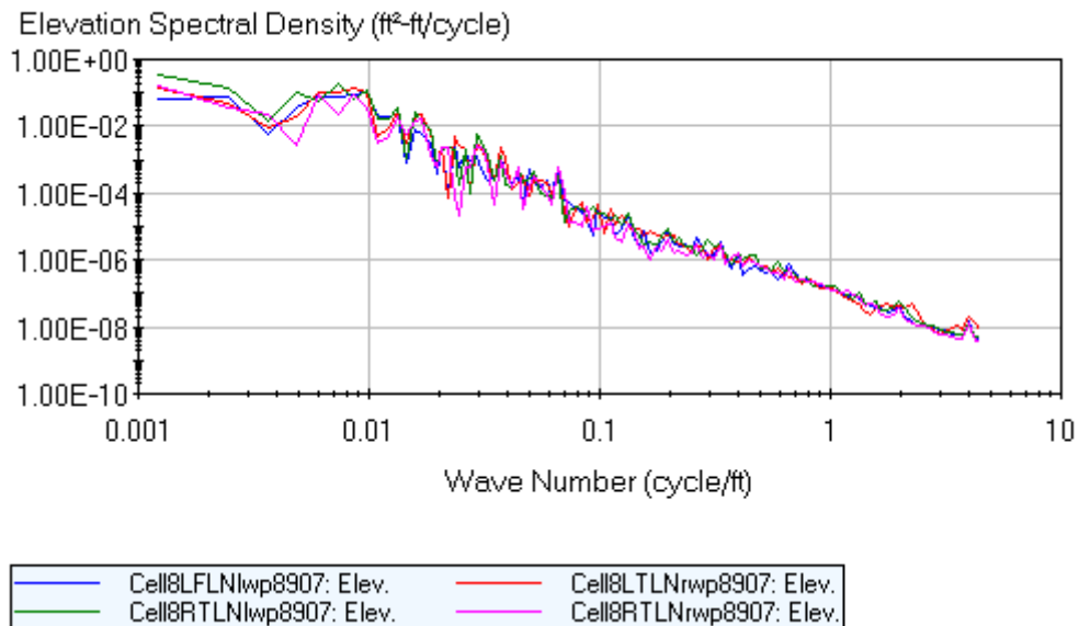
Figure B.4. Cell 8 pre-grind wave number.
