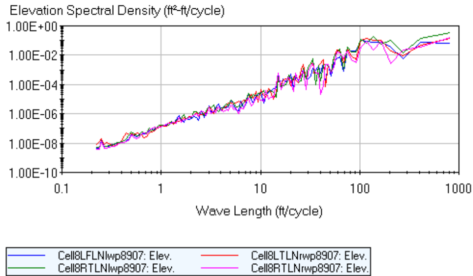
Figure B.5. Cell 8 pre-grind wavelength.
