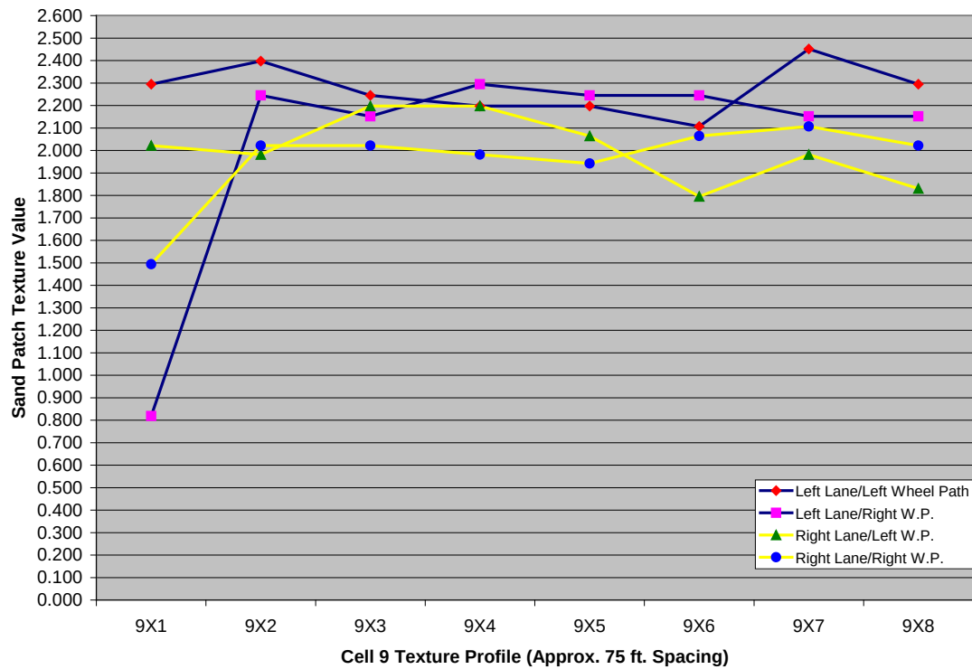
Figure 4.14. Sand volumetric technique ASTM E-965 test result on Cell 9.
