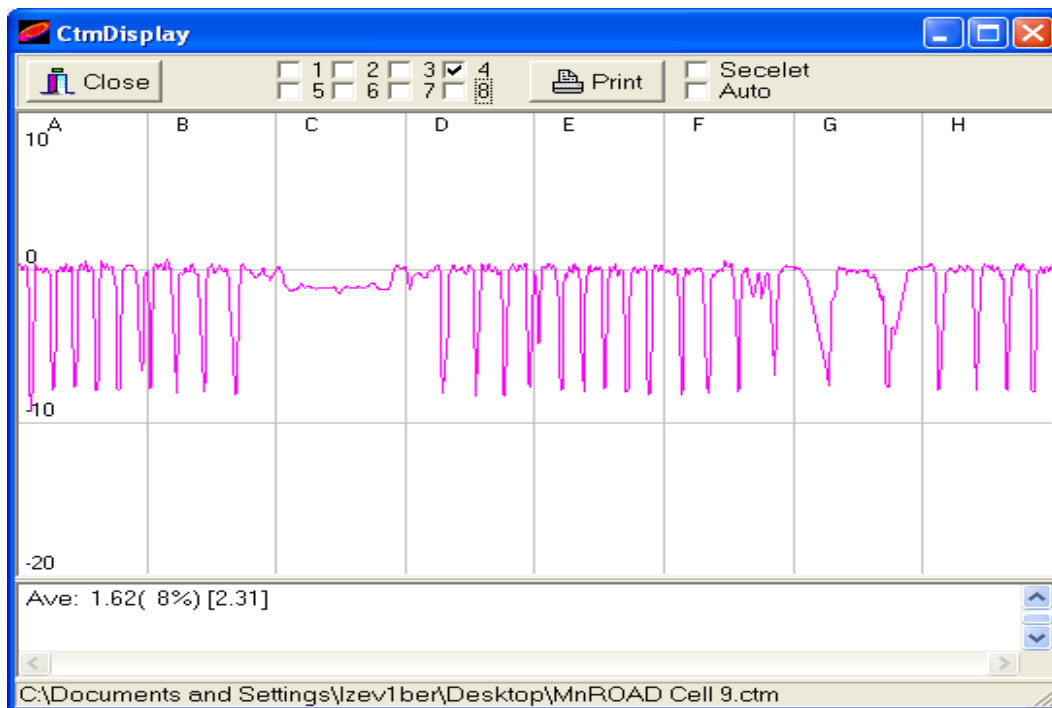
Figure 4.15. Screen capture of Ultimate Grind with CTM (ASTM E-2157).
