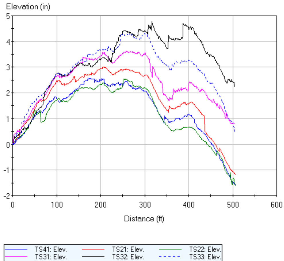
Figure F.1. Cell 37 pre-grind ride report.
