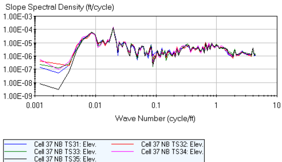
Figure F.6. Cell 37 post-grind wave number.
