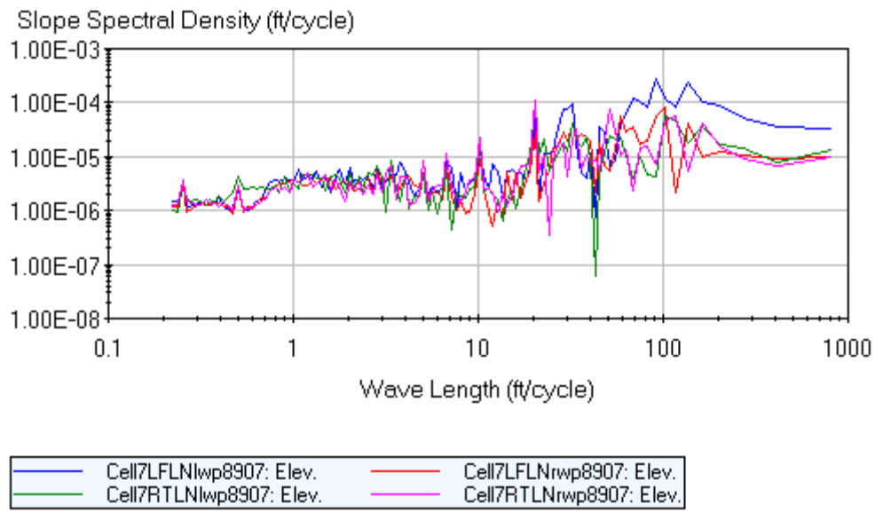
Figure B.2. Cell 7 pre-grind wavelength.
