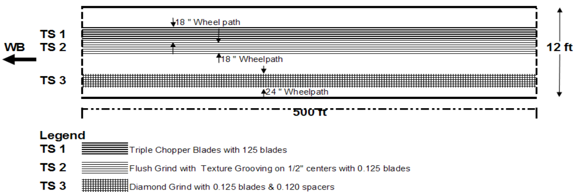
Figure 2.3. Diamond grinding test section layout on Cell 37.
