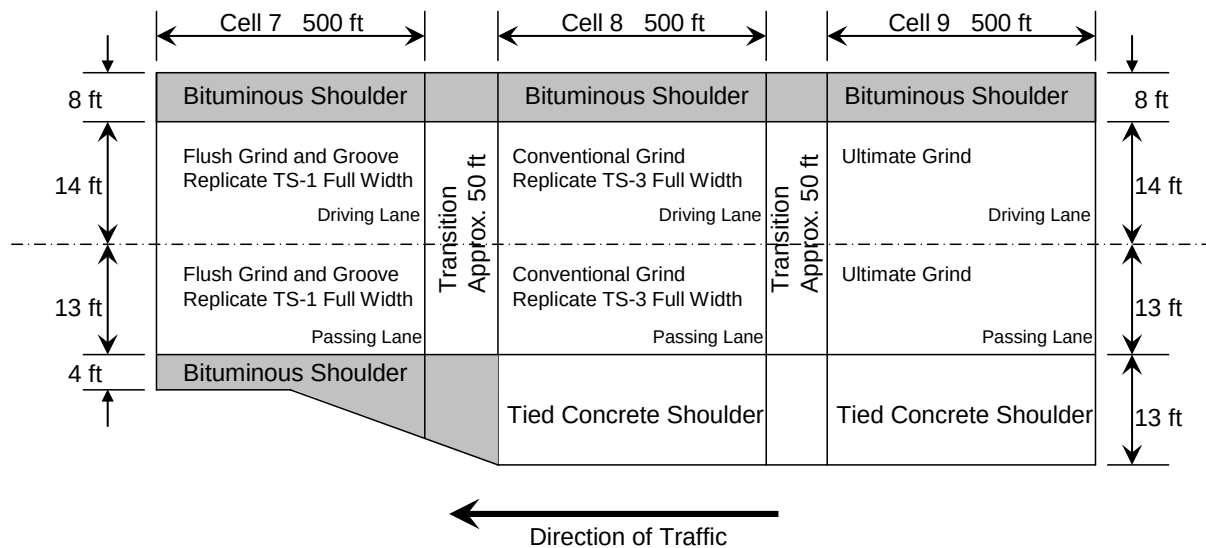
Figure 4.1. Layout of grinding activities – Cells 7, 8, and 9.
