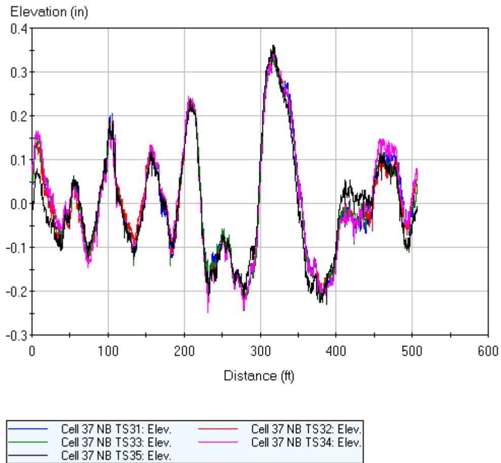
Figure F.5. Cell 37 pre-grind report (tested 6/18/07).
