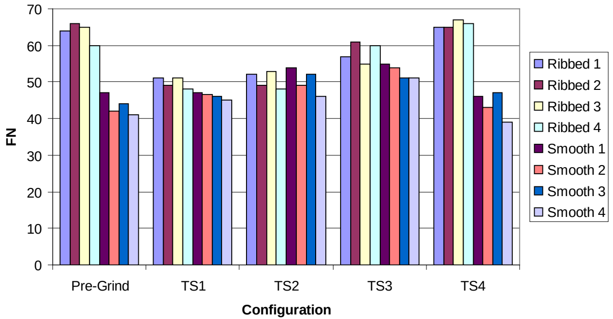
Figure F.8. Cell 37 friction.
