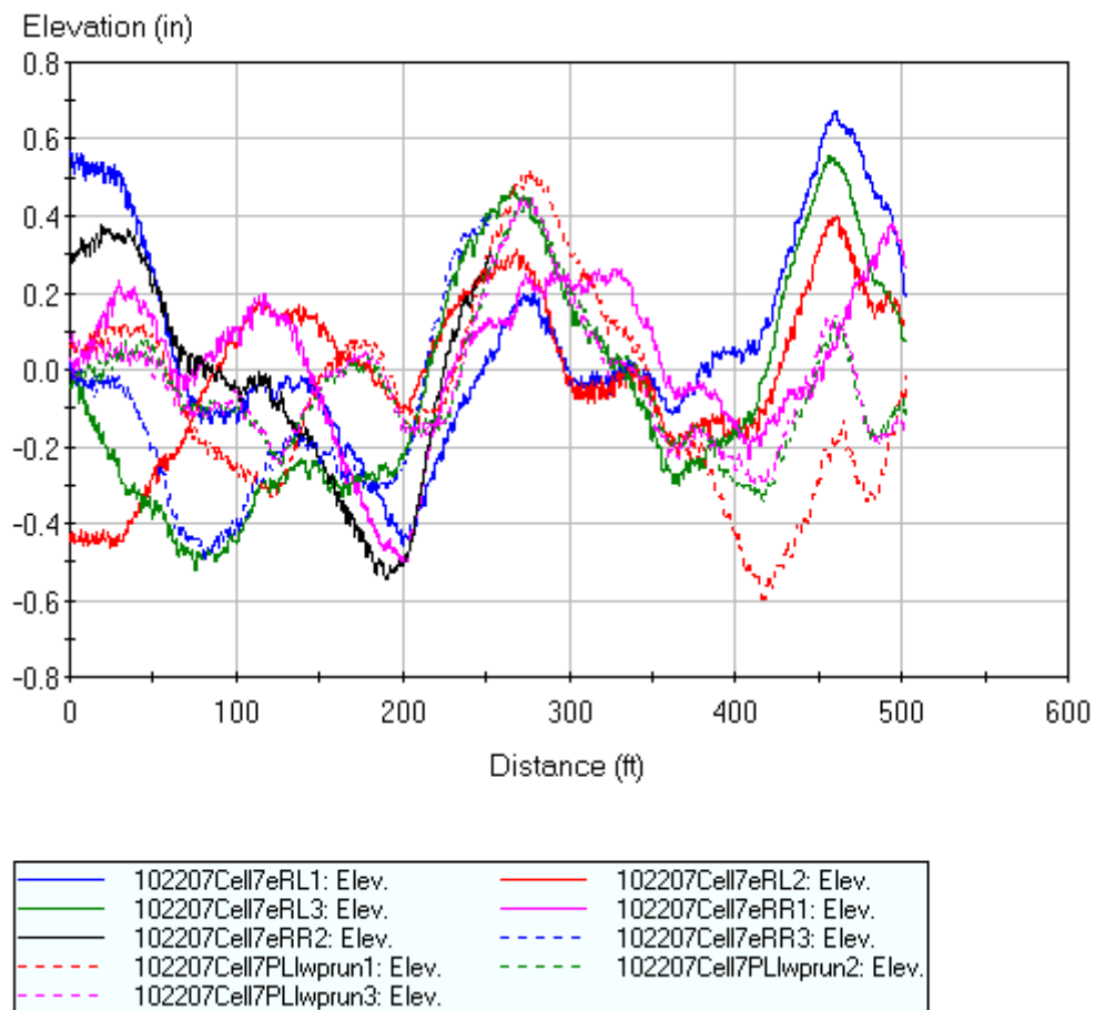
Figure B.6. Cell 7 post-grind ProVAL report.
