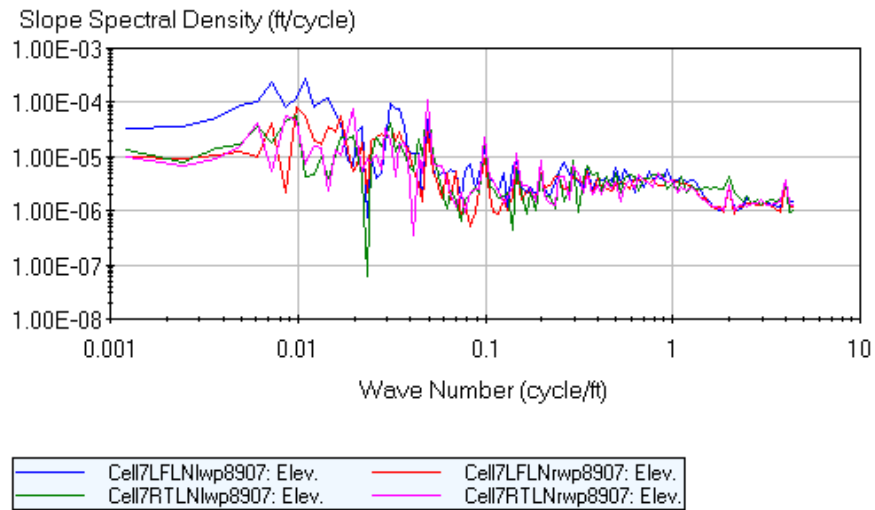
Figure B.1. Cell 7 pre-grind wave number.
