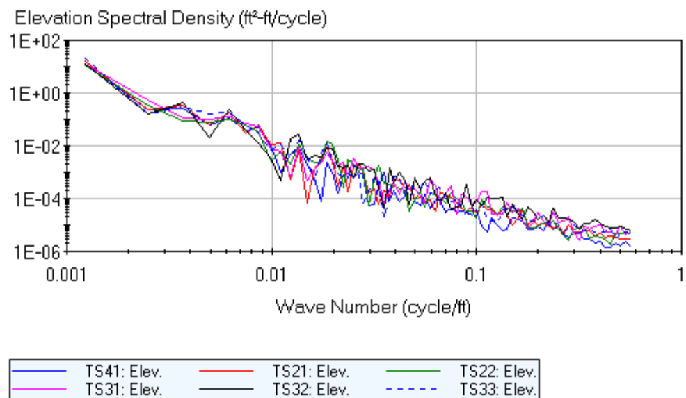
Figure F.2. Cell 37 pre-grind wave number.
