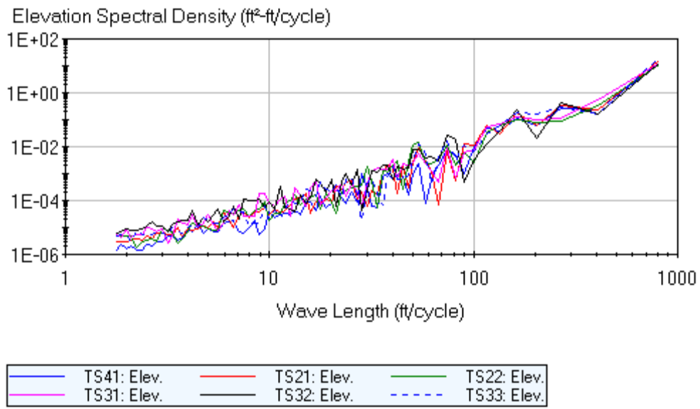
Figure F.3. Cell 37 pre-grind wavelength.
