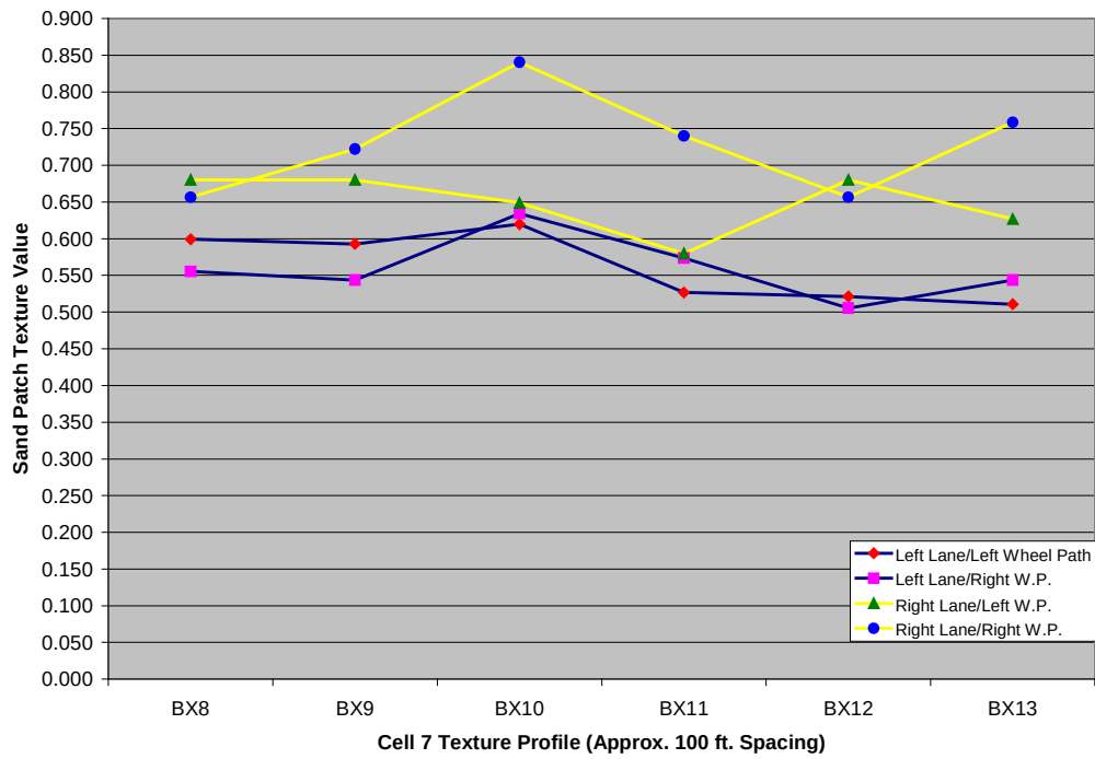
Figure 4.12. Sand volumetric technique ASTM E-965 test result on Cell 7.
