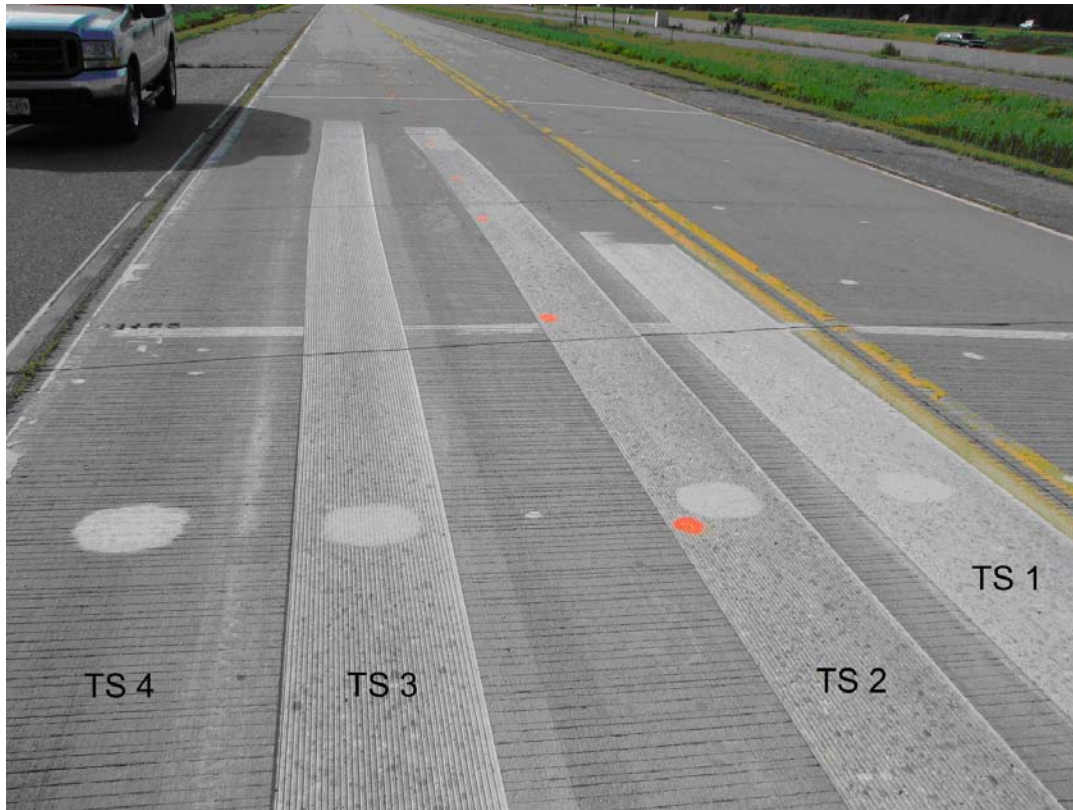
Figure 2.6. Grinding configurations in Cell 37, looking westbound.
