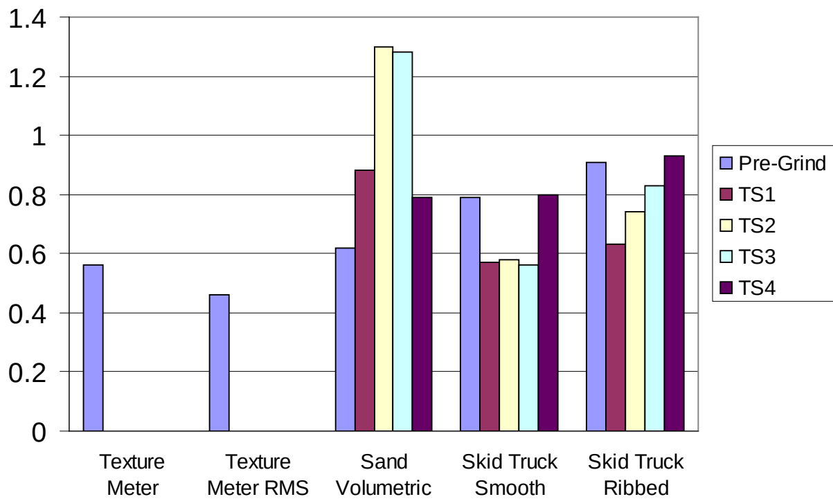
Figure F.4. Variability of post-grind texture with measurement procedure.
