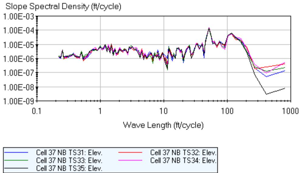
Figure F.7. Cell 37 post-grind wavelength.
