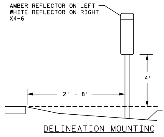
TYPICAL RURAL DESIGN
