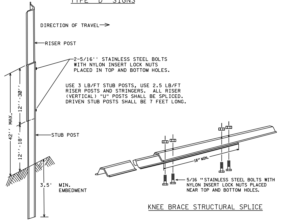
"U" POST BREAKAWAY SPLICE
