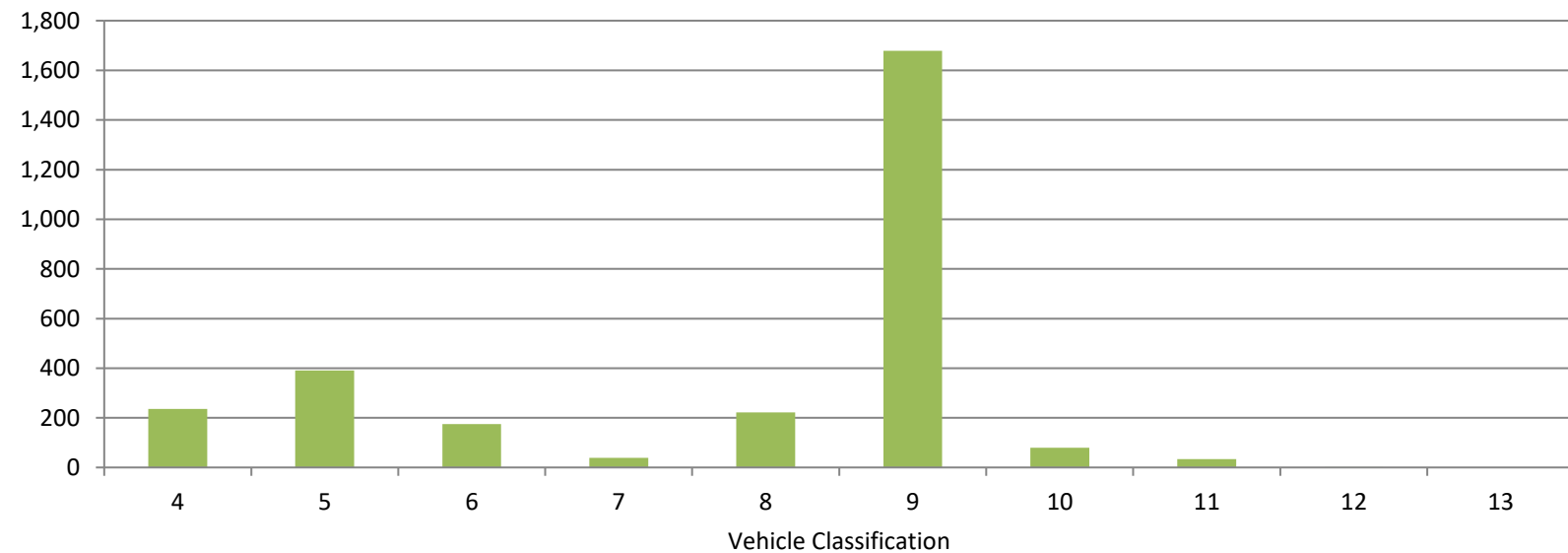
ATR 382 Heavy Commercial Average Daily Volume
