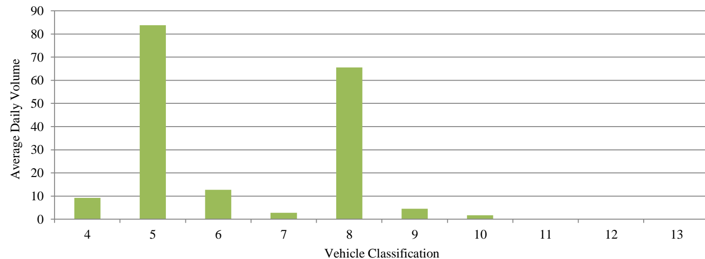
ATR 458 Vehicle Distribution
