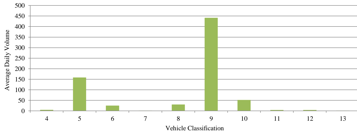
WIM 33 Vehicle Distribution
