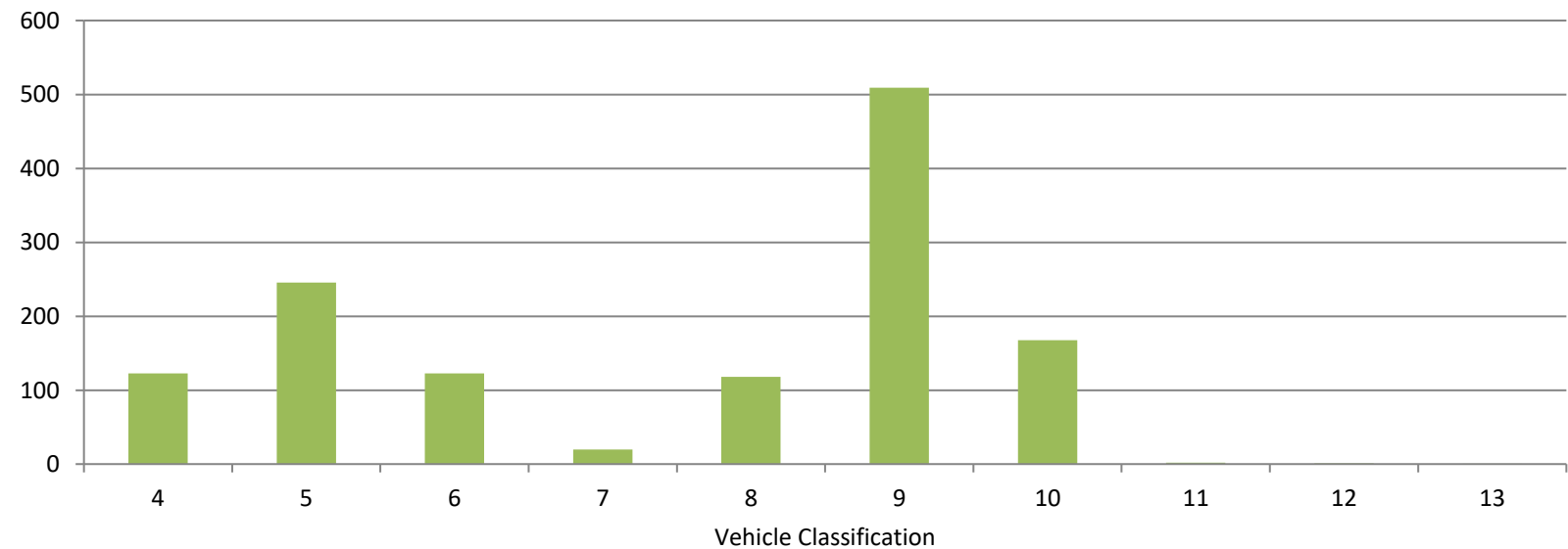
ATR 351 Heavy Commercial Average Daily Volume
