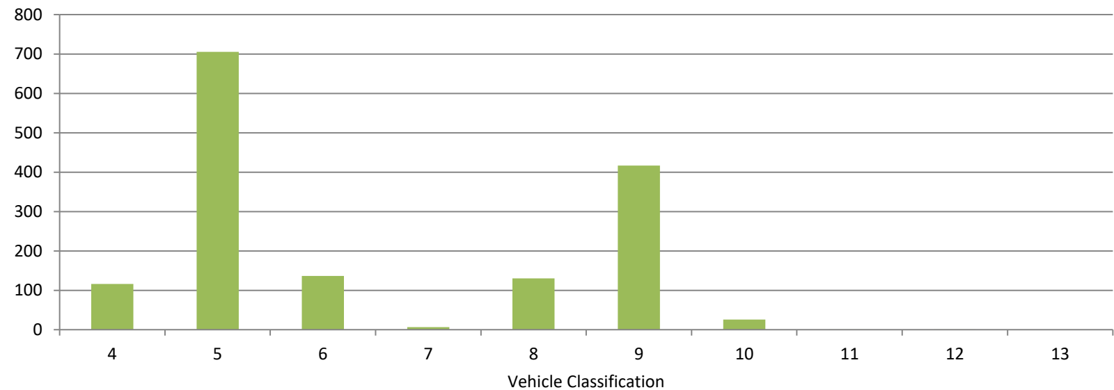
ATR 384 Heavy Commercial Average Daily Volume
