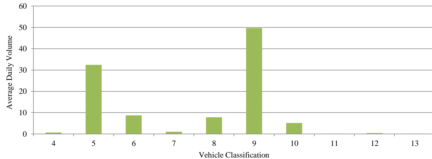
WIM 46 Vehicle Distribution
