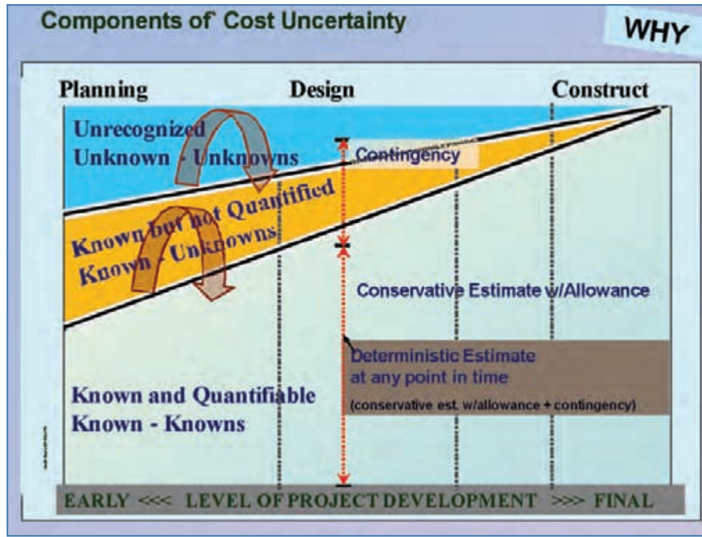
Figure 3.5 WSDOT Components of Cost Certainty
