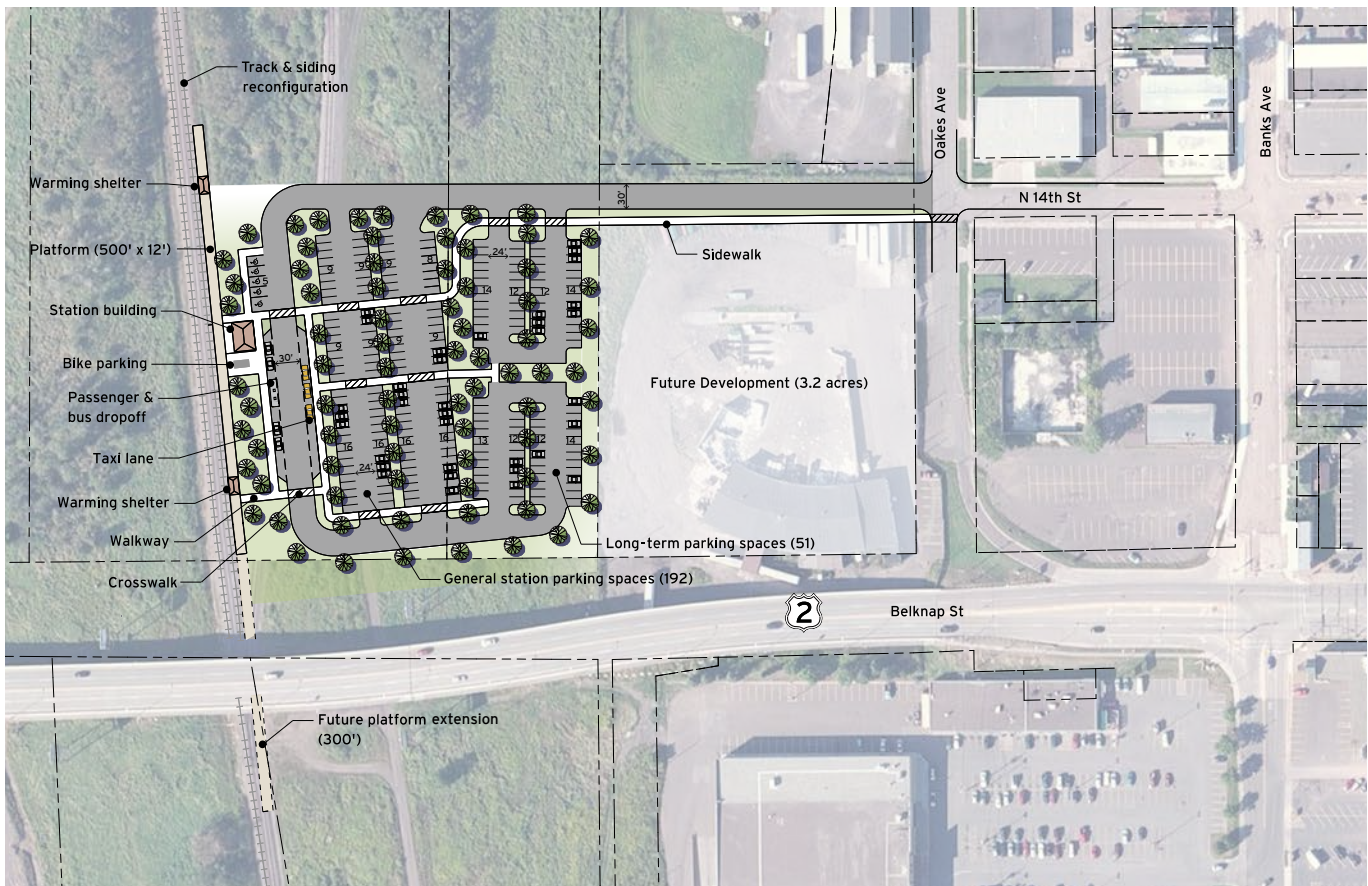
Conceptual layout of the Superior station
