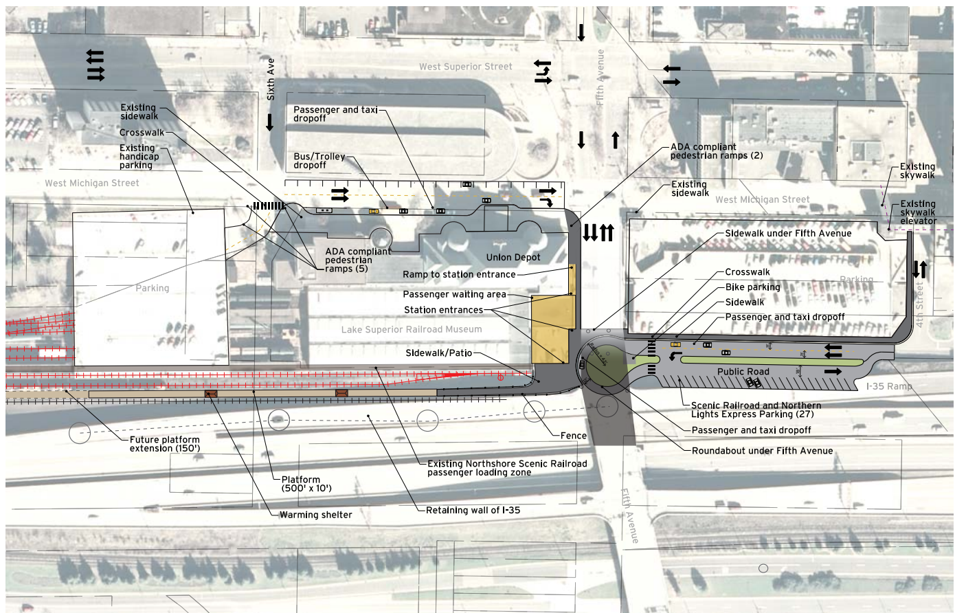
Conceptual layout of the Duluth station
