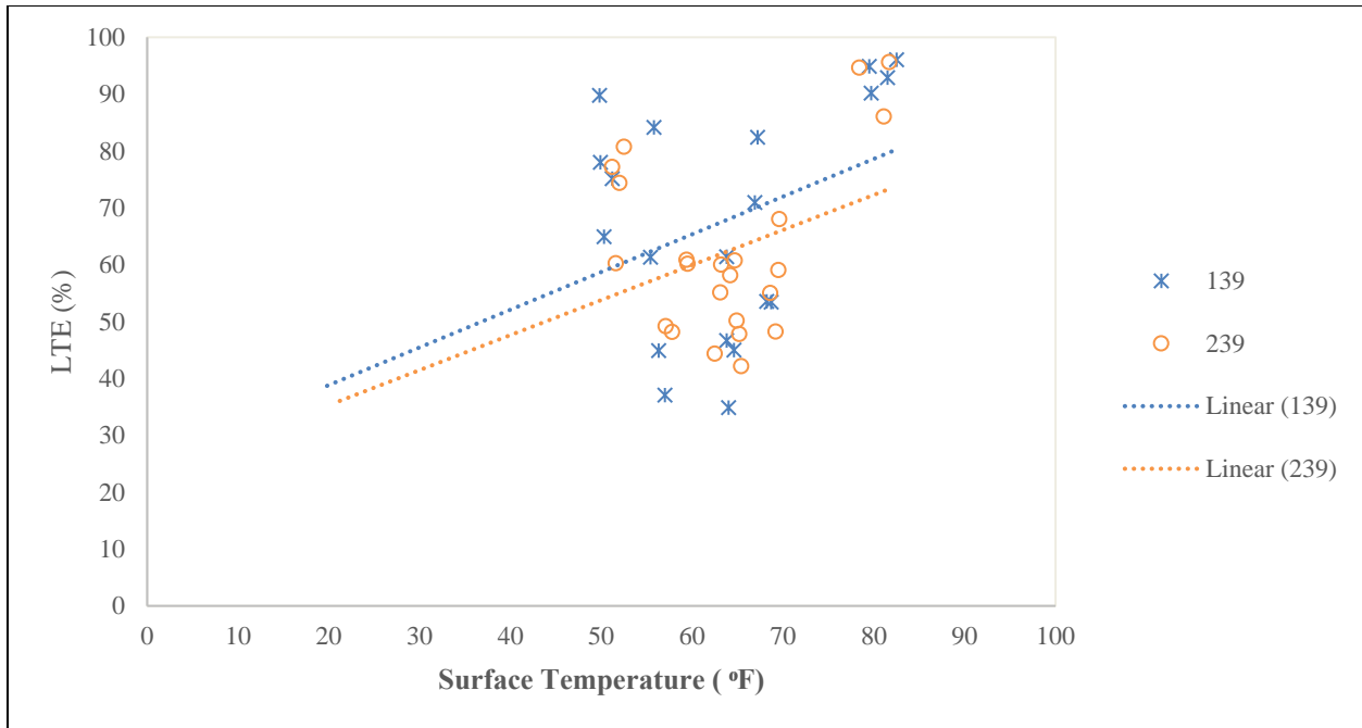
Figure 5-94: LTE vs. Pavement surface temperature for Cells 139 and 239.
