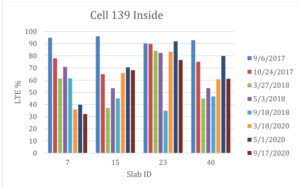
Figure 5-43. LTE of Cell 139 inside lane.
