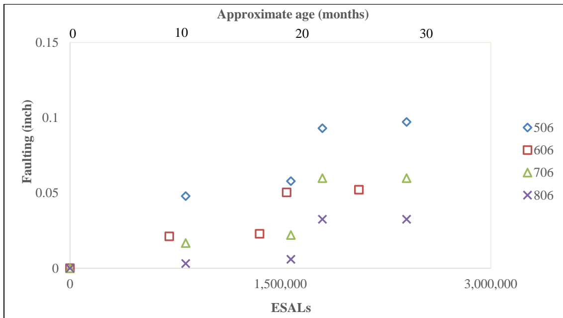
Figure 4-10: Faulting vs. ESALs for Cells 506,606,706 & 806.
