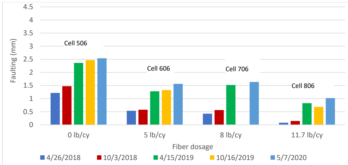
Figure 4-4. Faulting for Cells 506 through 806 with respect to fiber dosage (a) Only driving lane joints (b) average of the driving and passing lane joints.
