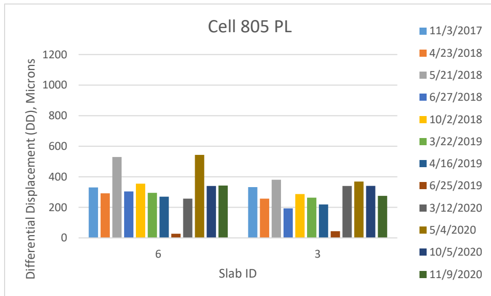
Figure 5-74. Differential displacement of Cell 805 passing lane.
