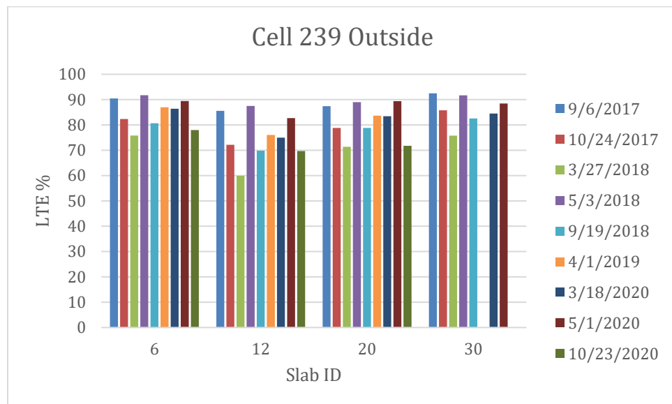
Figure 5-46. LTE of Cell 239 outside lane.
