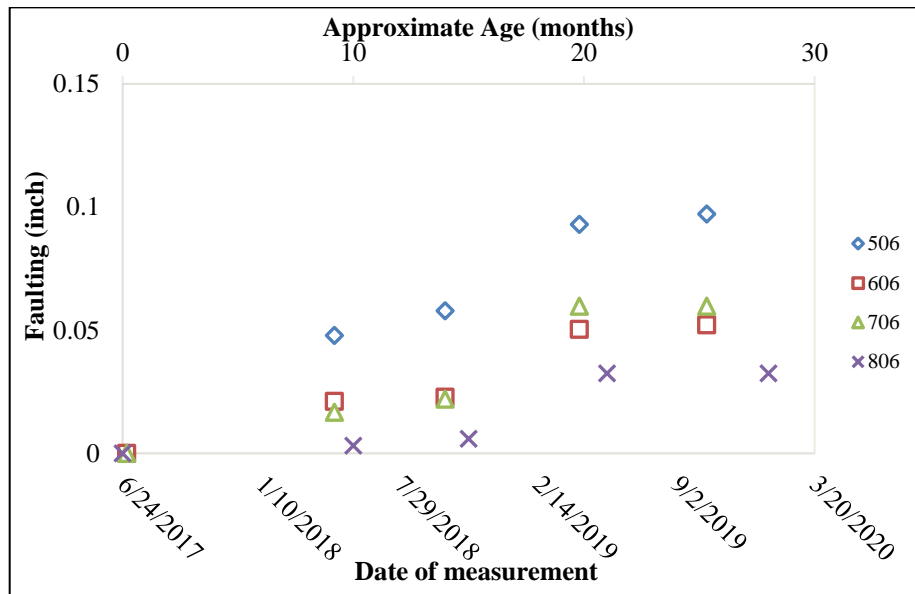
Figure 4-7: Faulting vs. Age for Cells 506,606,706 & 806.
