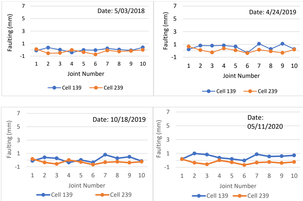
Figure 4-1. Faulting summary of Cells 139 and 239 at four different dates until May 11, 2020.
