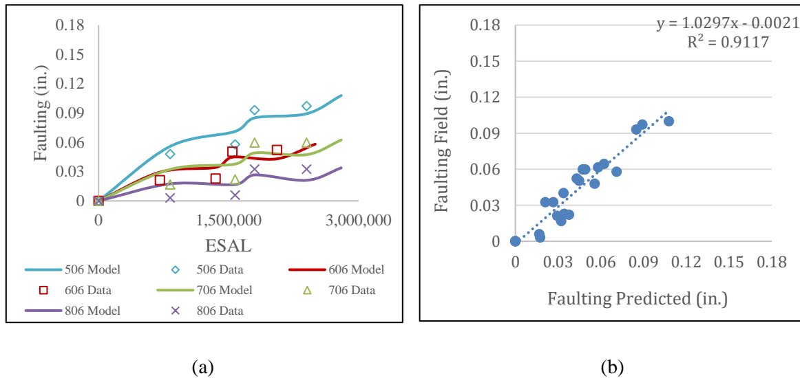
Figure 4-13: (a) Comparison of the measured faulting and predicted faulting, (b) Predictability of the proposed faulting prediction equation.
