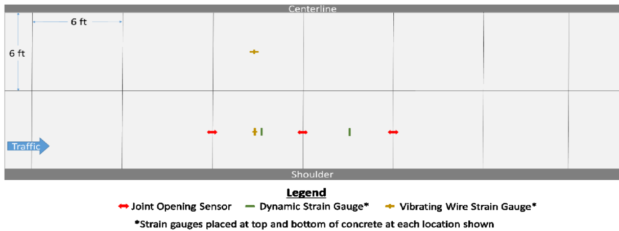
Figure A- 5. Sensor plan for Cell 506, driving lane (MnDOT, 2018).
