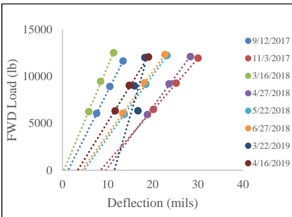
Figure 5-92: Deflection vs FWD load for (a) Cell 506 (b) Cell 806
