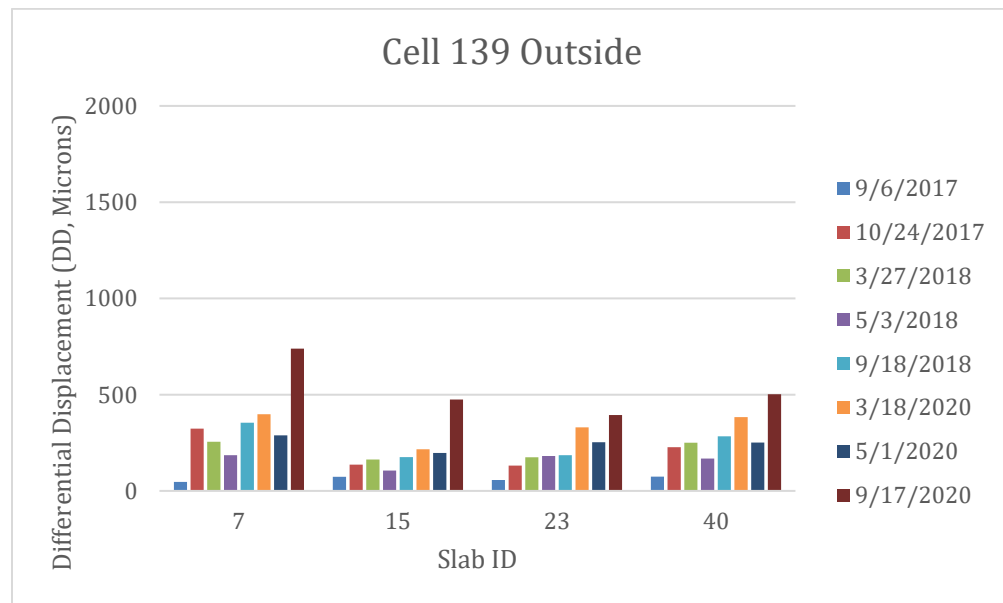
Figure 5-60. Differential displacement of Cell 139 outside line.
