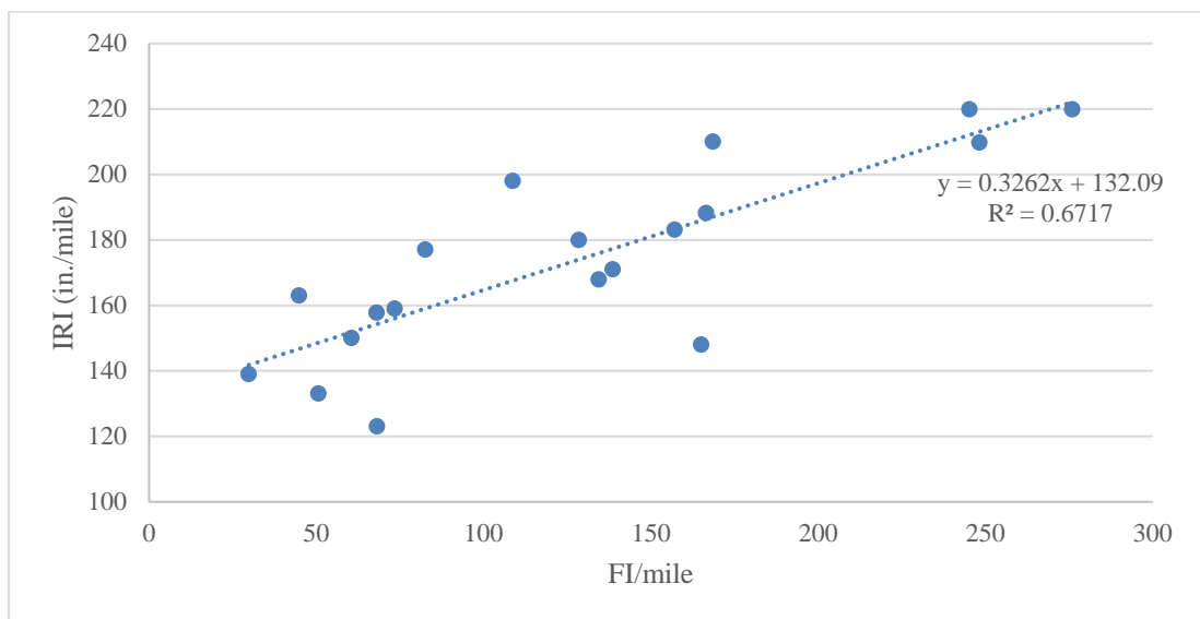
Figure 4-19: Correlation between IRI and faulting index.
