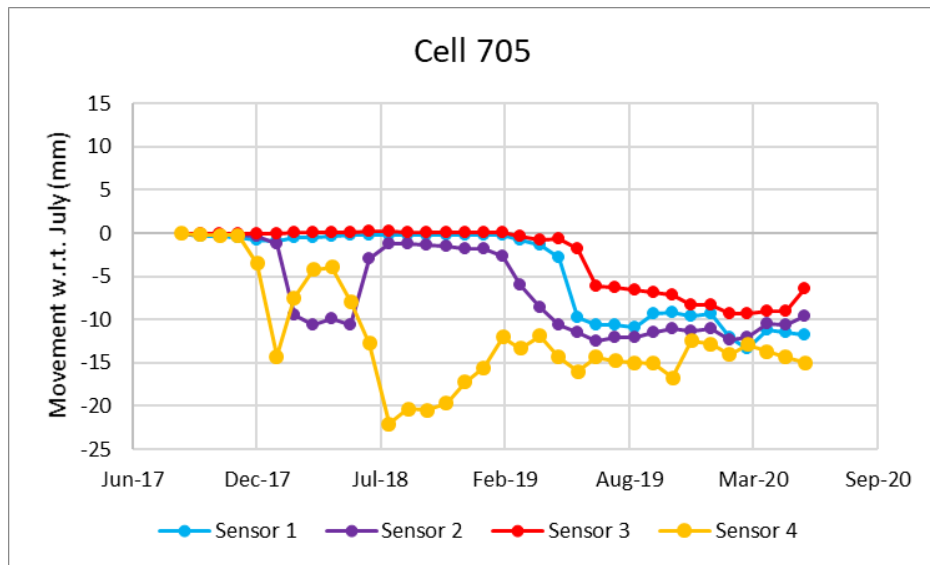
Figure 5-41. Monthly average relative joint movement for Cell 705.
