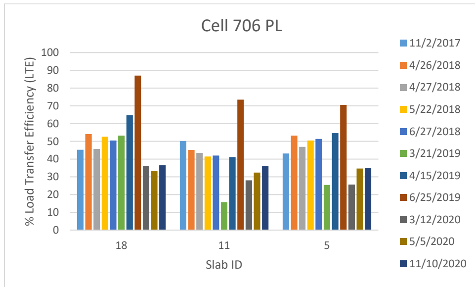
Figure 5-52. LTE of Cell 706 passing lane.
