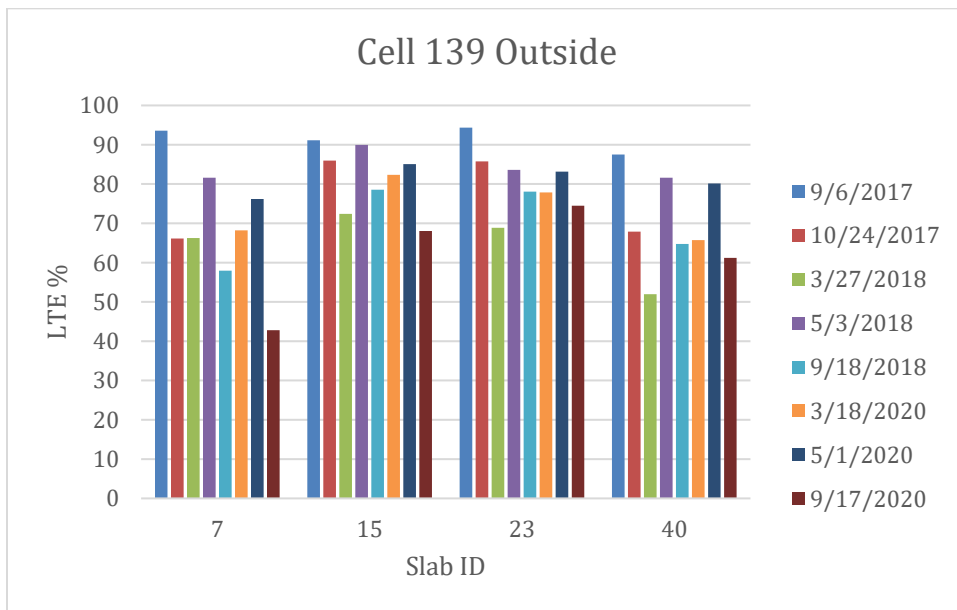
Figure 5-44. LTE of Cell 139 outside lane.
