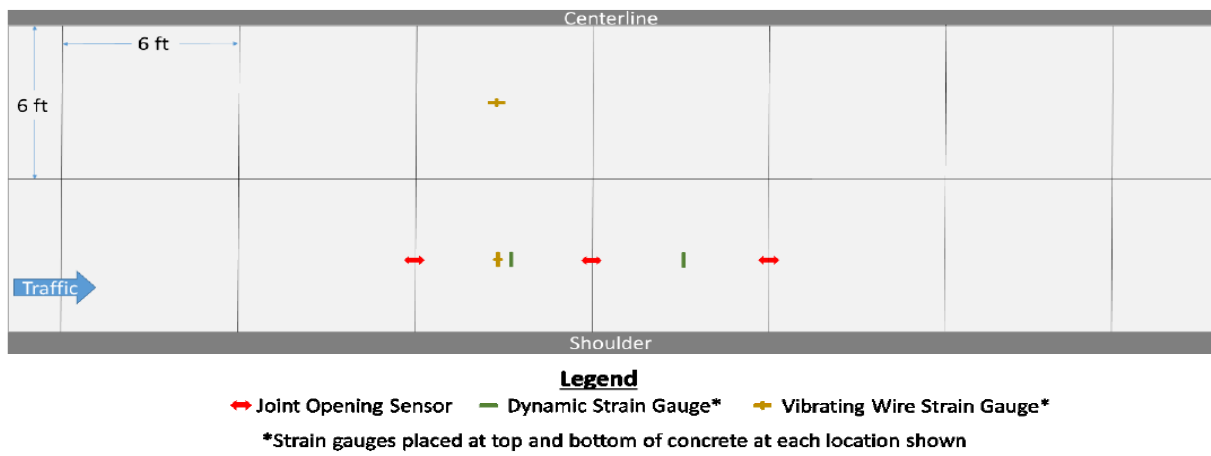
Figure 2-4: Sensor plan for Cell 506, driving lane.
