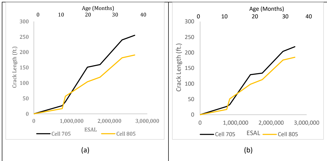
Figure 3-36. Crack Length vs ESAL for Cells 705 and 805 (a) Driving and Passing lane combined (b) Driving Lane only.
