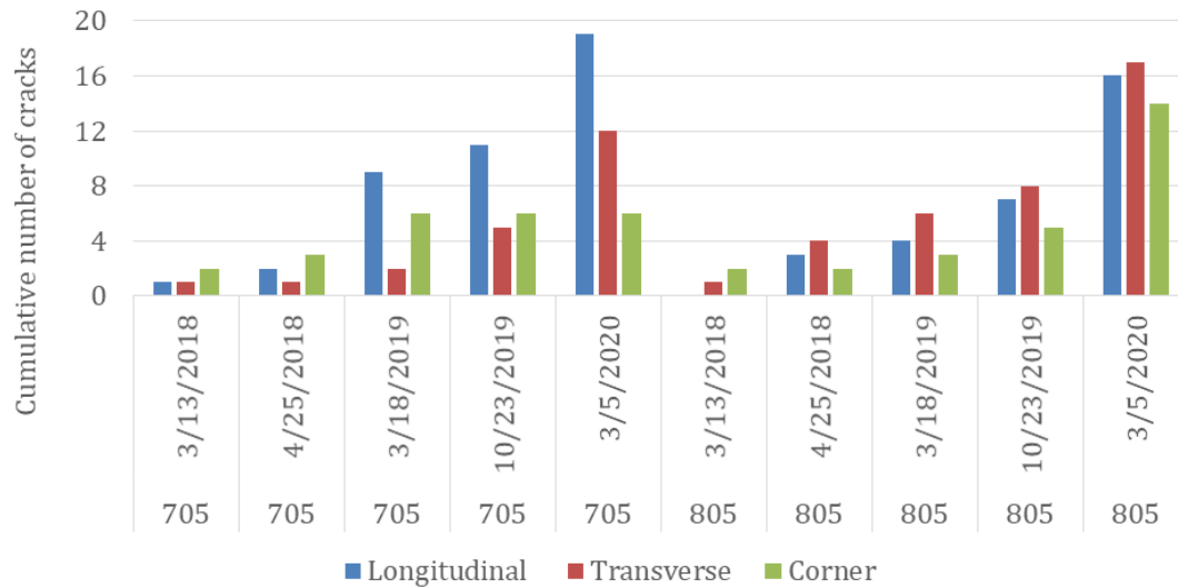
Figure 3-28. Cumulative number of various cracks in Cell 705 and 805.
