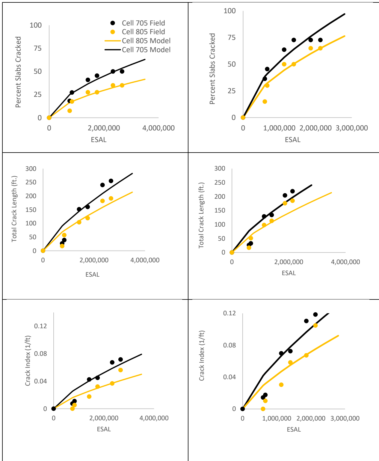
Figure 3-39. Correlation between the fatigue crack parameters and ESAL for 5 inches thick concrete overlays.
