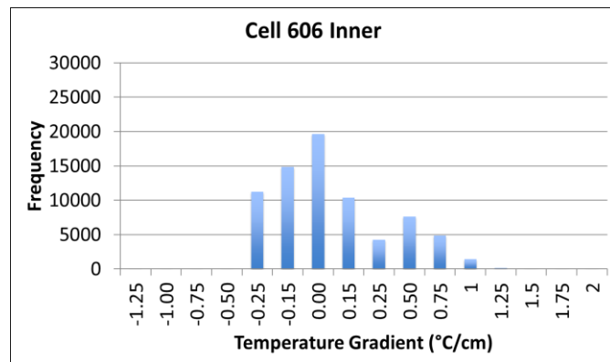
Figure 5-13. Frequency distributions of the linear temperature gradient for various cells.
