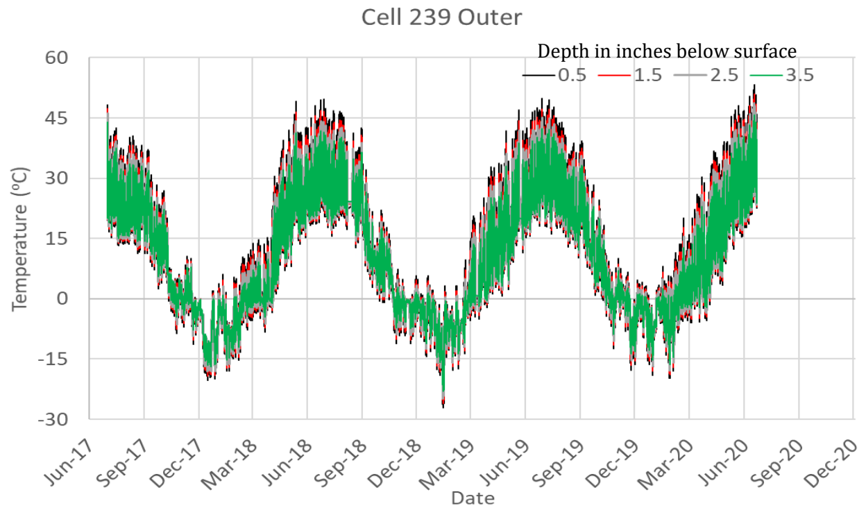
Figure 5-5. Temperature profile of Cell 239 outer lane.
