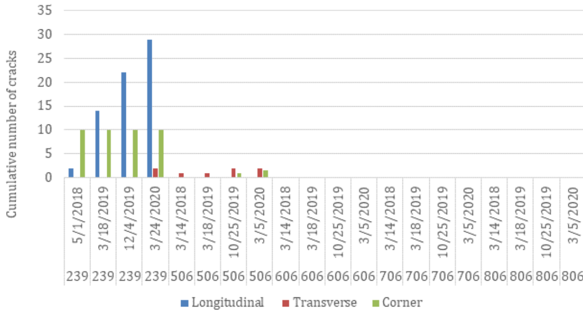
Figure 3-16: Summary of fatigue cracks of cells on gravel base until March 2020 (Cell 139 not shown).
