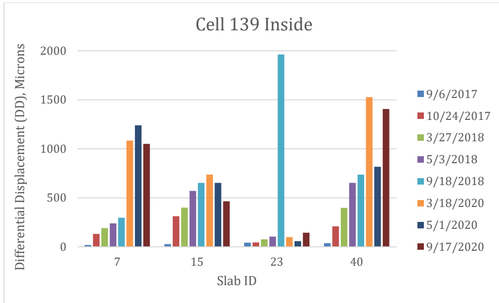
Figure 5-59. Differential displacement of Cell 139 inside line.
