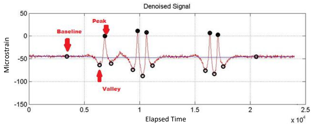
Figure 2-8. An example of a plot of strain due to the dynamic load exerted by the MnDOT truck.
