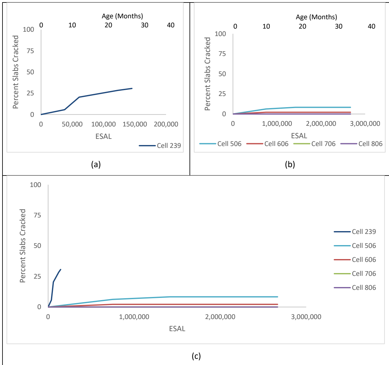
Figure 3-30: Percentage Crack vs. ESAL for the driving lane only (a) 239 (b) 506,606,706, and 806 (c) 239, 506, 606, 706, and 806.
