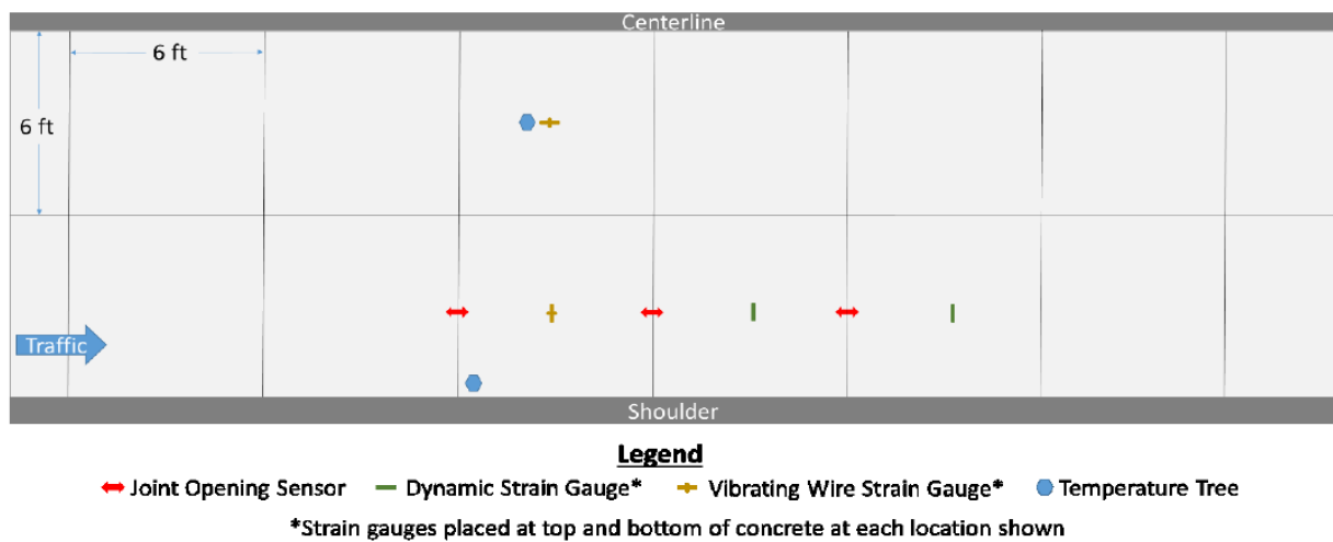
Figure A- 6. Sensor plan for Cell 606, driving lane.
