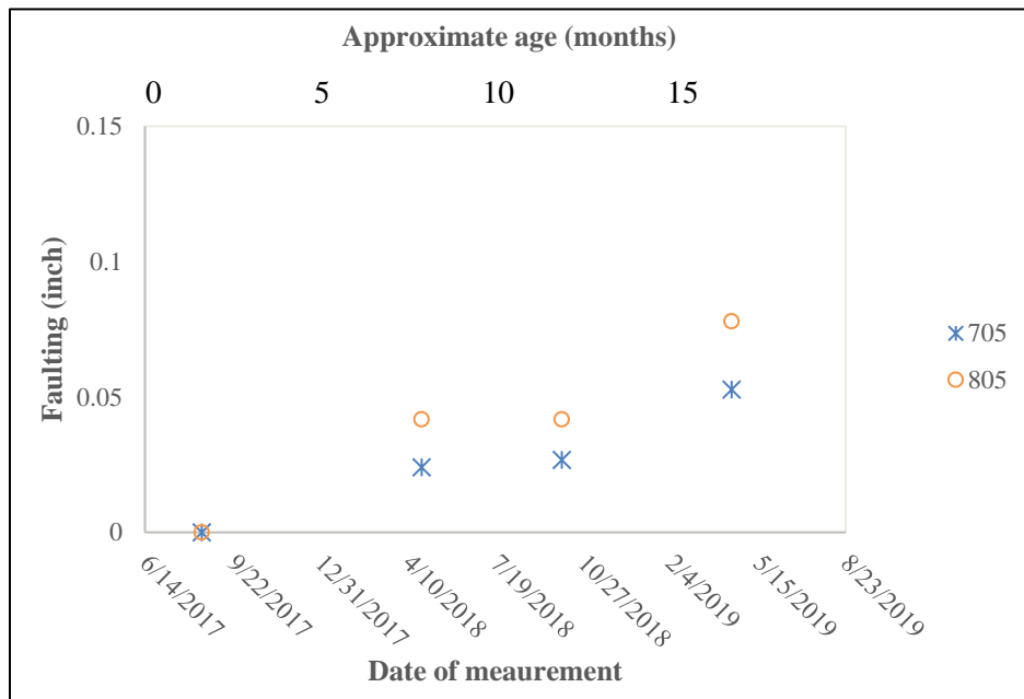
Figure 4-8: Faulting vs. Age for Cells 705 & 805.
