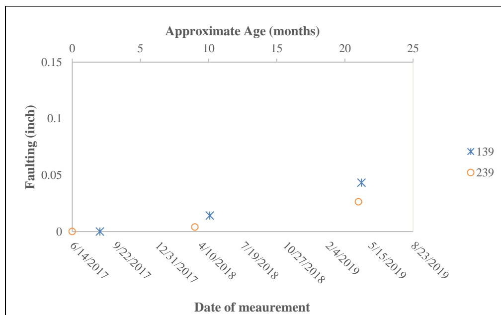
Figure 4-6. Faulting vs. Age for Cells 139 & 239.
