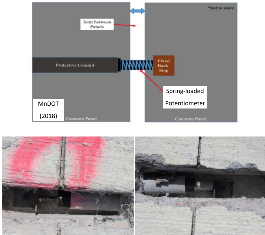
Figure 2-9. Sketch and photographs of joint opening sensors before installation of protective covering.
