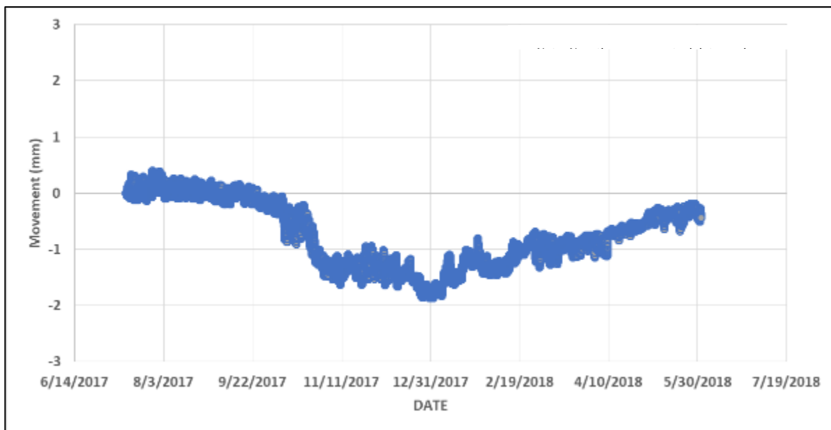
Figure 5-34. Movement recorded by Sensor 3 of Cell 706; no adjustment was required. (Note diff. scale in y-axis).
