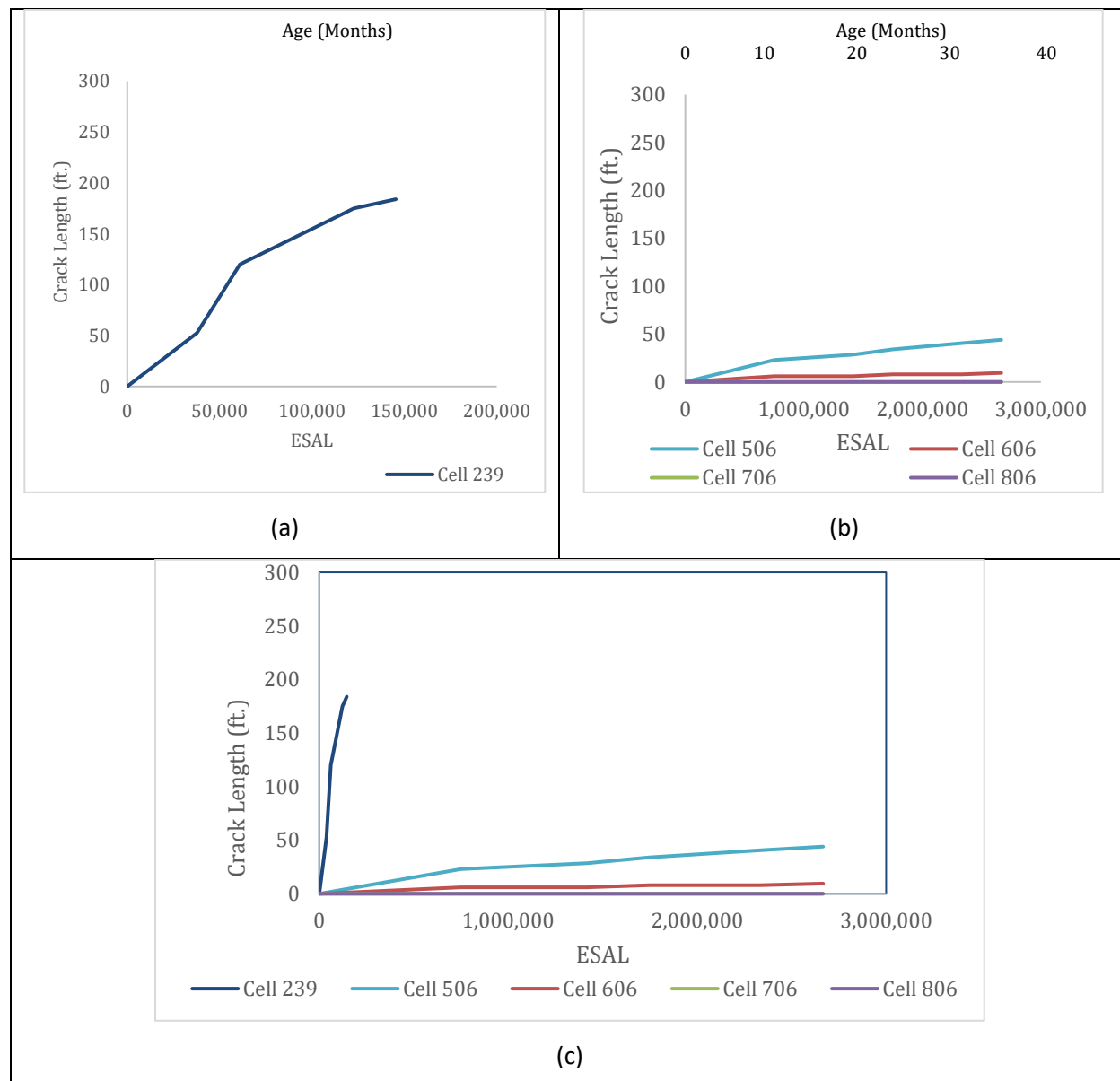
Figure 3-31: Crack Length vs. ESAL for both lanes (a) 239 (b) 506,606,706, and 806 (c) 239, 506, 606, 706, and 806
