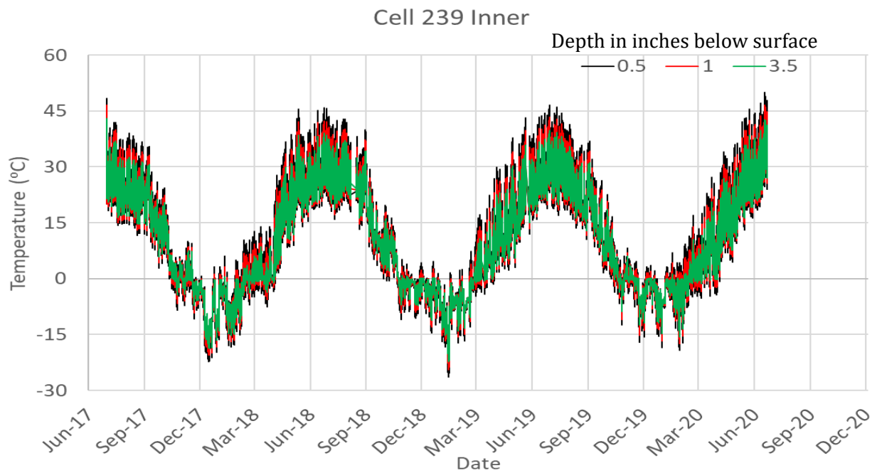
Figure 5-4. Temperature profile of Cell 239 inner lane.
