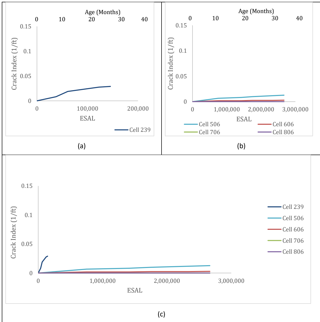
Figure 3-33: Crack Index vs. ESAL for both lanes (a) 239 (b) 506,606,706, and 806 (c) 239, 506, 606, 706, and 806.
