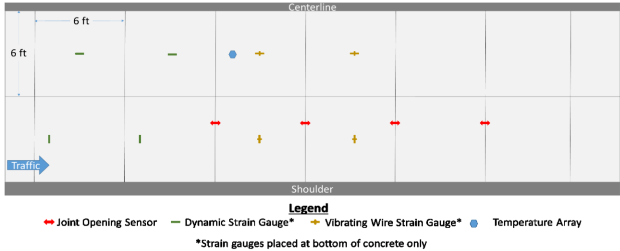
Figure 2-3: Sensor plan for Cell 139 inner lane.
