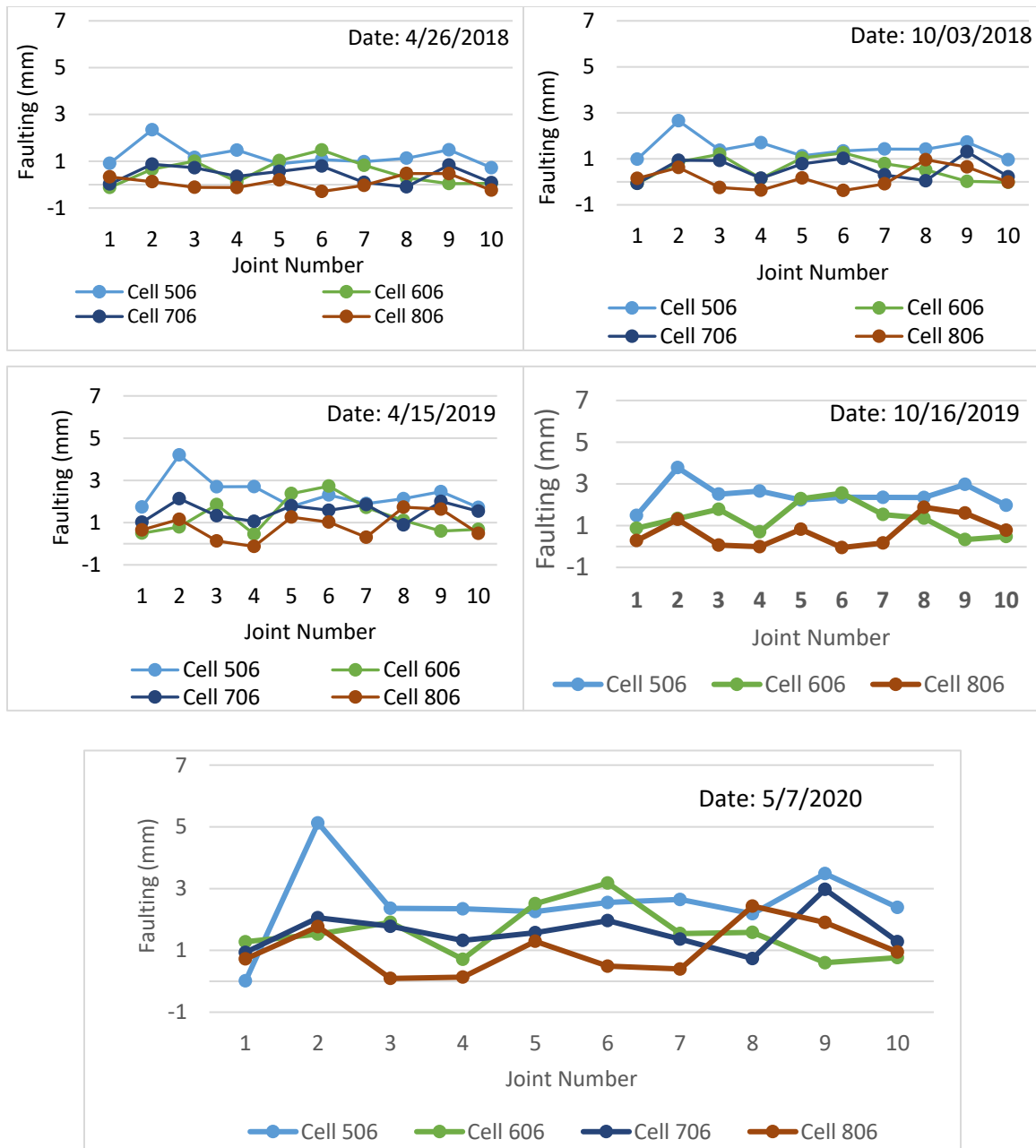
Figure 4-2. Faulting summary of Cells 506 through 806 until May 2020.
