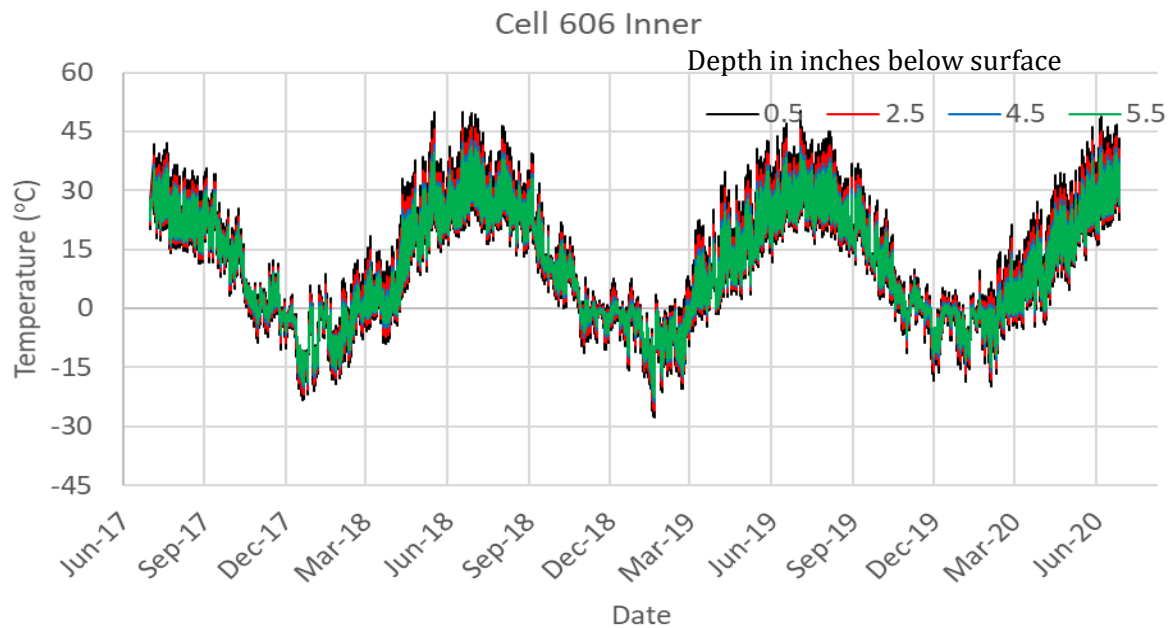
Figure 5-8. Temperature profile of Cell 606 inner lane.
