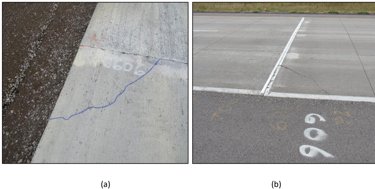
Figure 3-13. Corner crack (construction issue) in the last panel of Cell 606 observed (a) in the year 2018 and (b) 2019.
