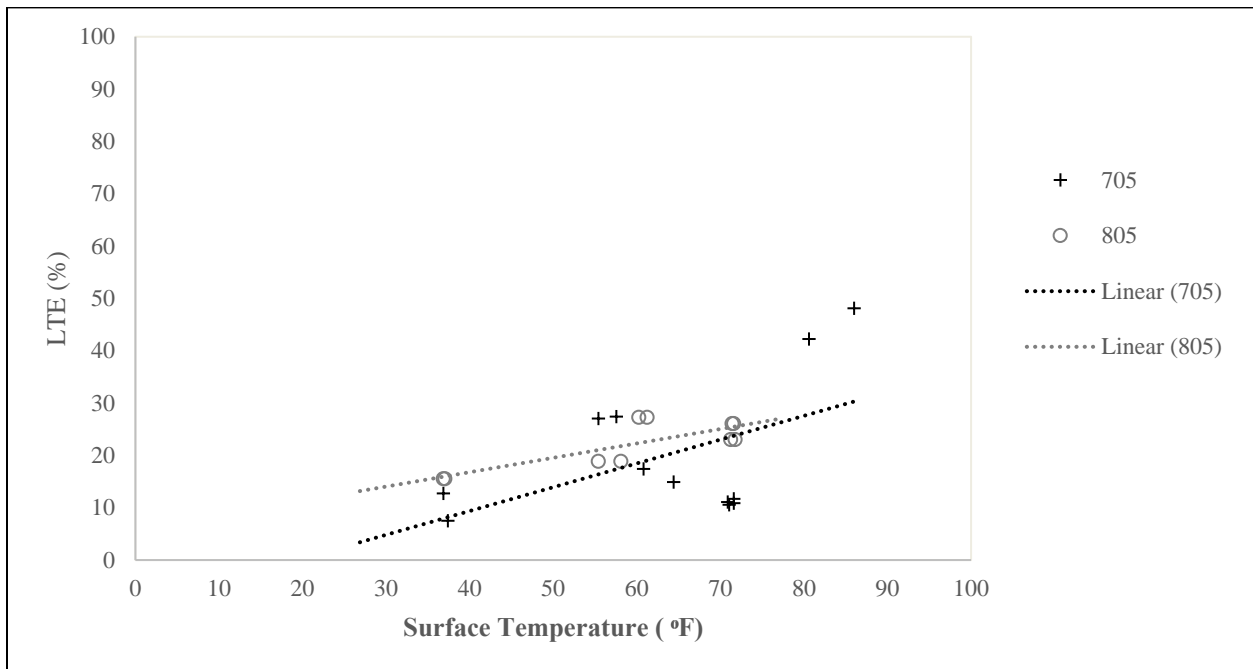
Figure 5-95: LTE vs. Pavement surface temperature for Cells 705 and 805.
