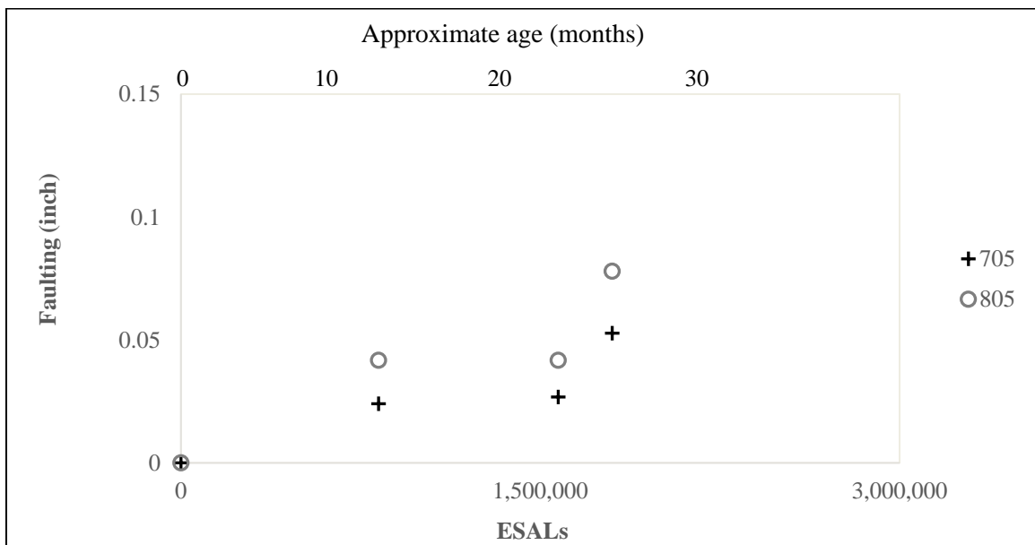
Figure 4-12: Faulting vs. ESALs for Cells 705 & 805.
