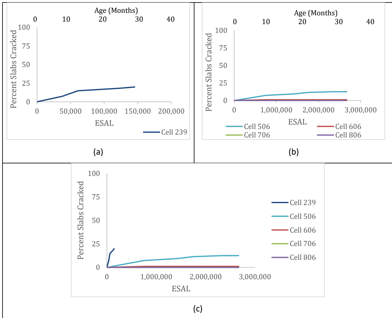
Figure 3-29: Percentage Crack vs. ESAL for both lanes (a) 239 (b) 506,606,706, and 806 (c) 239, 506, 606, 706, and 806.
