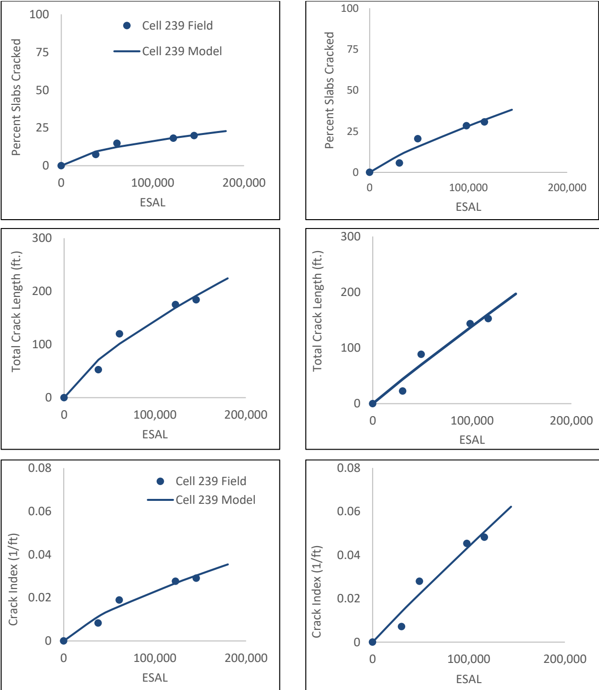
Figure 3-38. Correlation between the fatigue crack parameters and ESAL for Cell 239 (ultra-thin pavement). Plots on the left are for both lanes, and the right-side plots are for the only driving lane.
