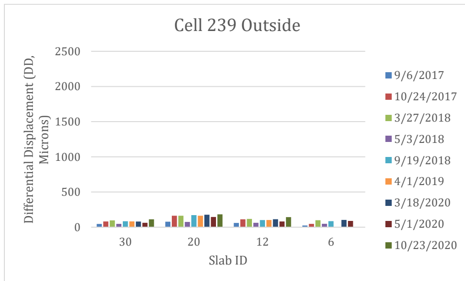
Figure 5-62. Differential displacement of Cell 239 outside line.
