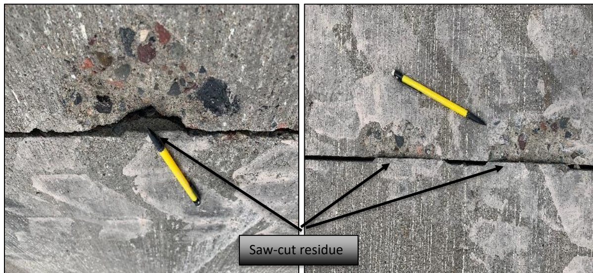
Figure 3-12. Hardened saw-cut residue found at the spalled joints of Cell 506.
