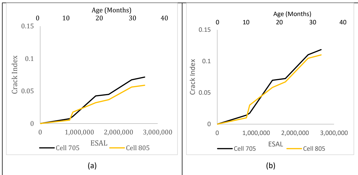
Figure 3-37. Crack Length vs ESAL for Cells 705 and 805 (a) Driving and Passing lane combined (b) Driving Lane only.
