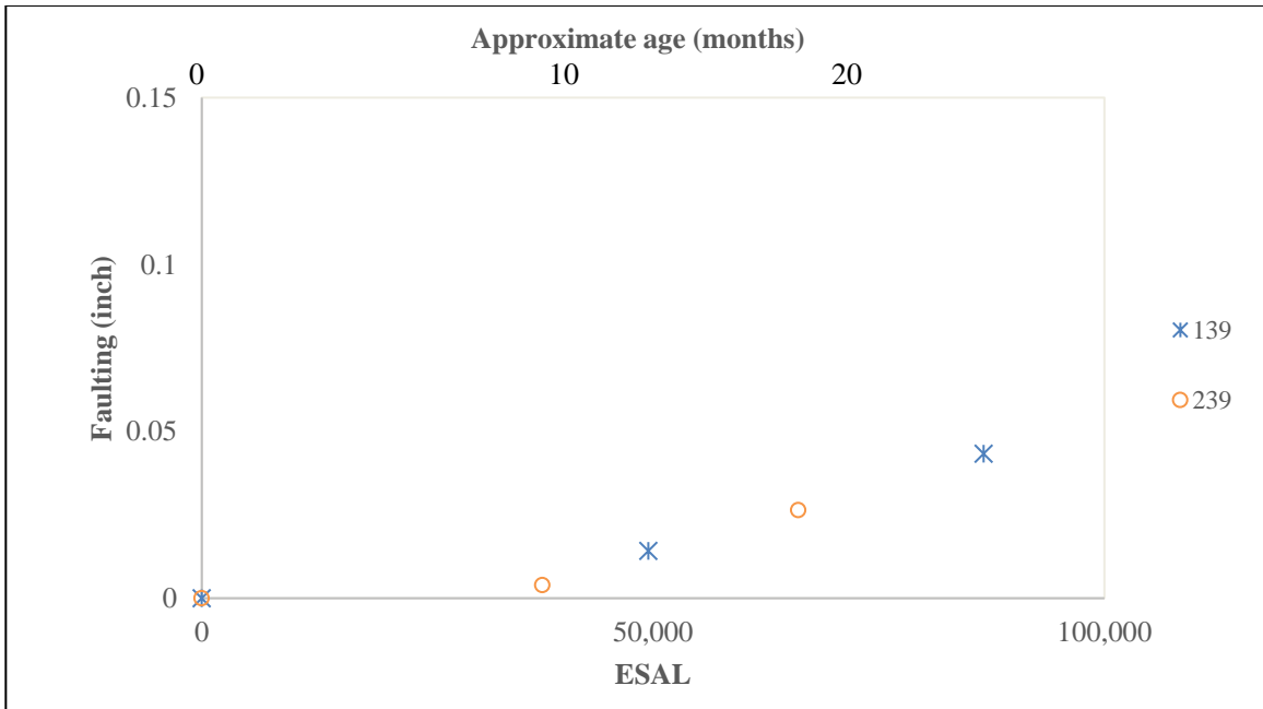
Figure 4-9: Faulting vs. ESALs for Cells 139 & 239.
