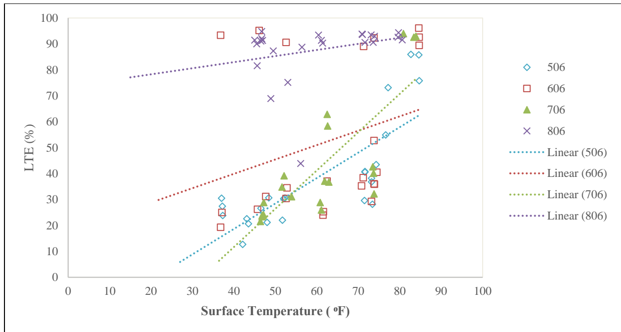
Figure 5-96: LTE vs. Pavement surface temperature for Cells 506, 606, 706 and 806.
