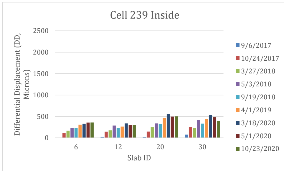
Figure 5-61. Differential displacement of Cell 239 inside line.
