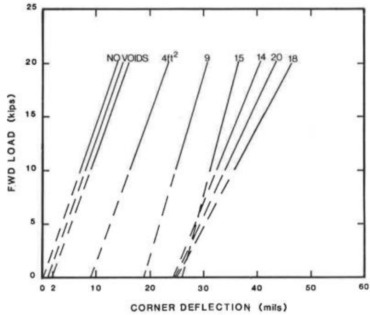
Figure 5-91: Use of FWD test data conducted at different load level to identify possible presence of voids (Crovetti and Darter, 1985)
