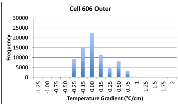
Figure 5-13. Frequency distributions of the linear temperature gradient for various cells.
