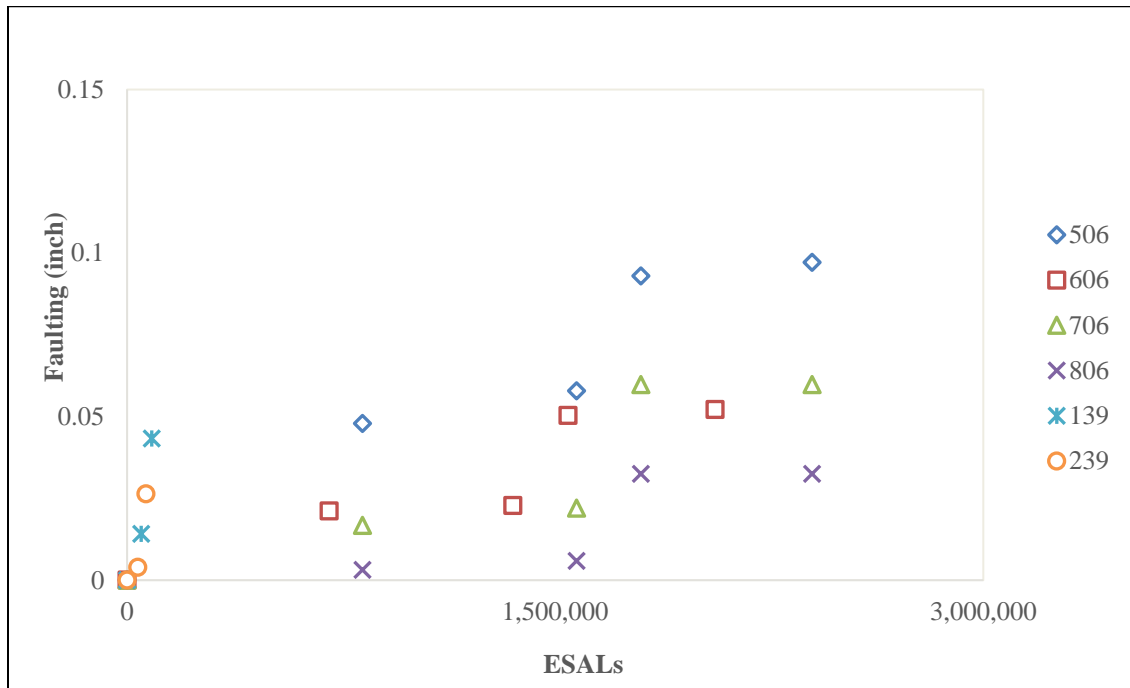
Figure 4-11: Comparison between low volume cells (139 and 239) and high-volume cells (506,606,706, and 806).
