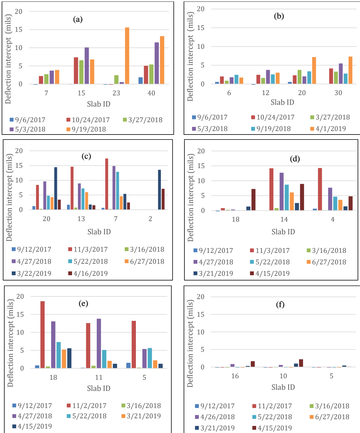
Figure 5-93: Deflection values under variable FWD load stresses for NRR test Cells (a) 139 (b) 239 (c) 506 (d) 606 (e) 706 and (f) 806.
