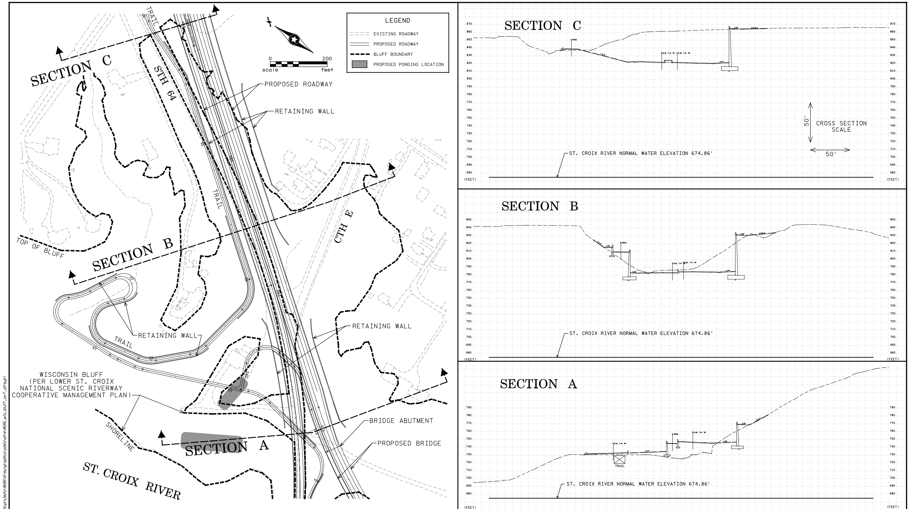
Wisconsin Bluff Cross Sections - Alternative E
