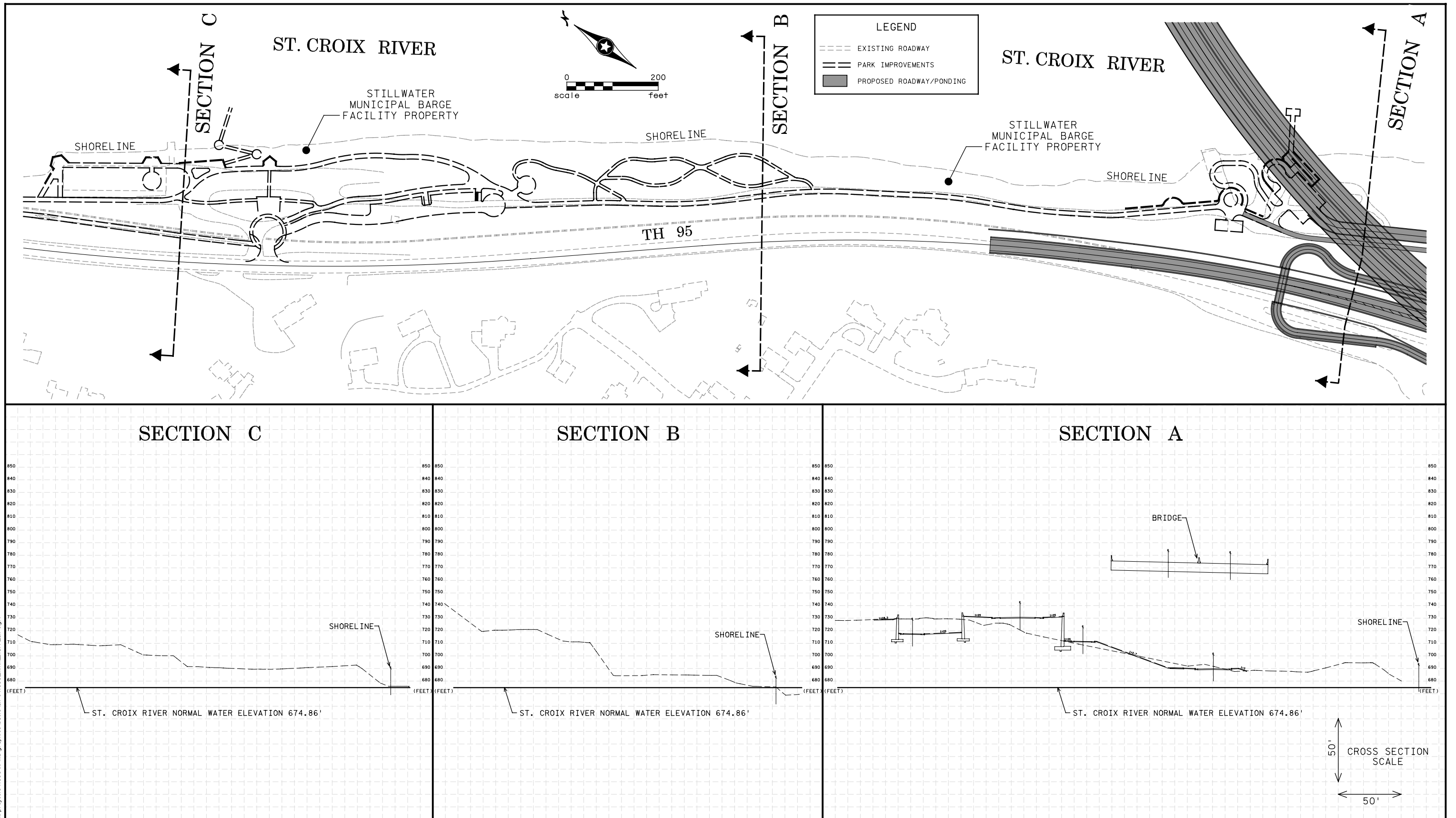
Minnesota Bluff Cross Sections - Alternative C
