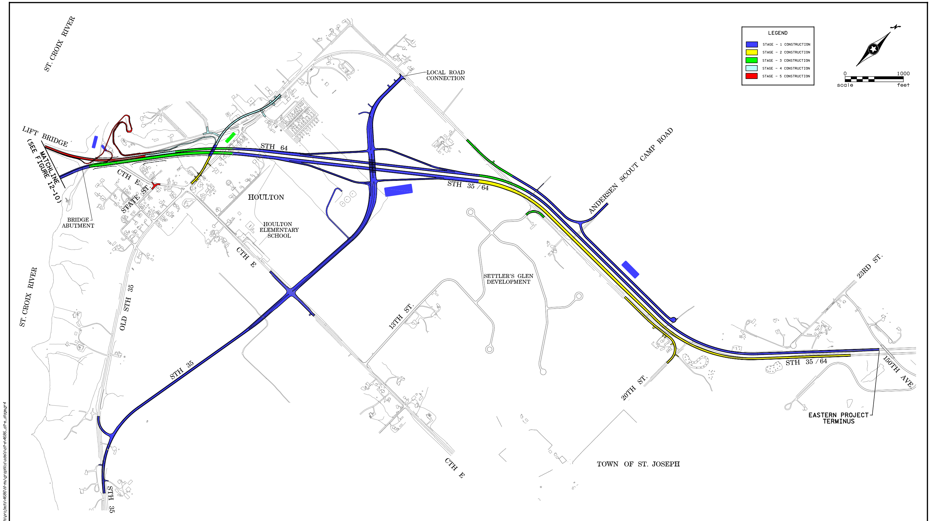
Wisconsin STH 35 / 64 - Staging Phase 1 (Alternative E)
