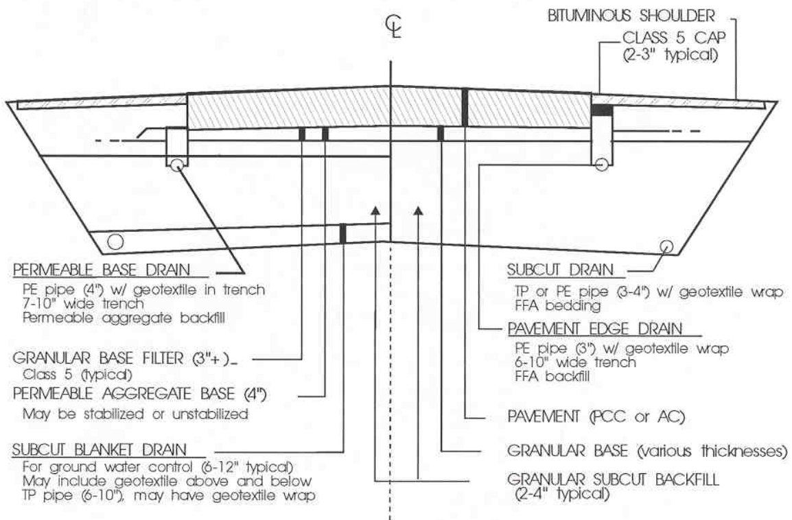
Figure 5-4.1. Typical sections, subsurface drainage.
