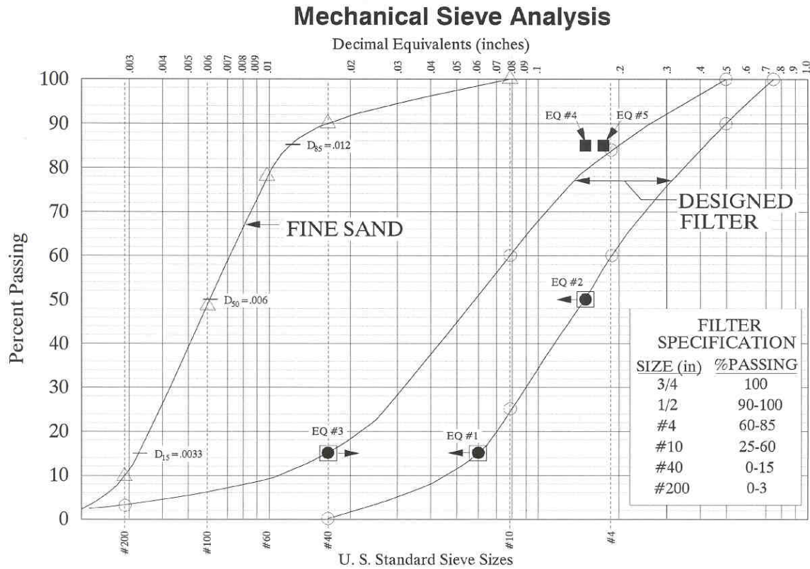
Figure 5-4.2 Granular Filter Calculations
