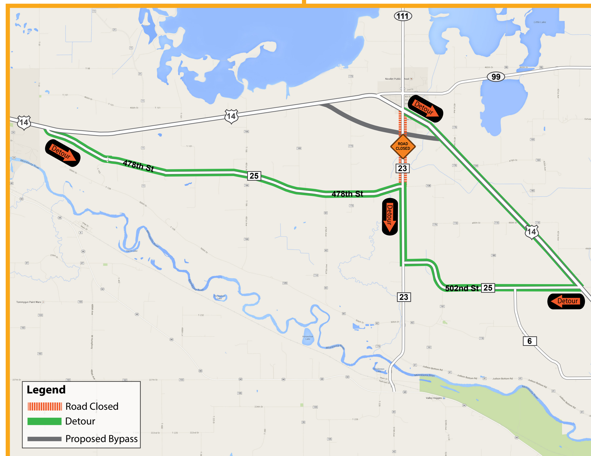
Bridge Construction, Roundabouts, Highway 111: CR 23 Detoured Route
