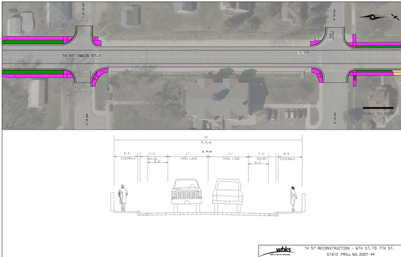
Typical Section 6 th Street to 7 th Street
