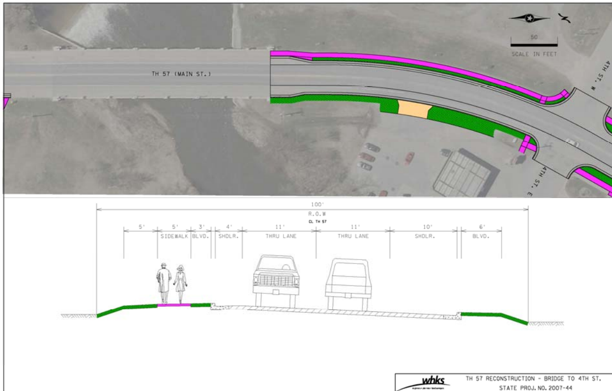
Typical Section Bridge to 4 th street
