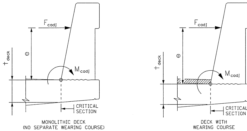
COLLISION LOADS ADJUSTED FOR BARRIER HEIGHT
