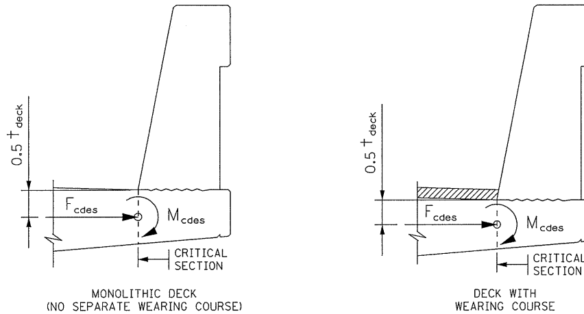
COLLISION LOADS FOR DESIGN
