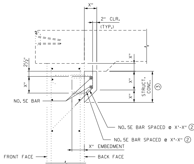
RECONSTRUCTED SECTION ④
