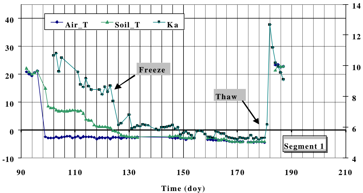
Figure 5 Temperature and Ka vs Time for TDR segment 1 (0-15cm). The Soil_T is the average temperature of the two thermocouples located at the top and bottom of the segment. Segment 1 went through a step-wise freezing cycle. Periodically a layer of insulation was removed and the temperature was allowed to stabilize. This can be seen between day 98 and 114. A rapid thaw gives a more distinct change in the Ka.
