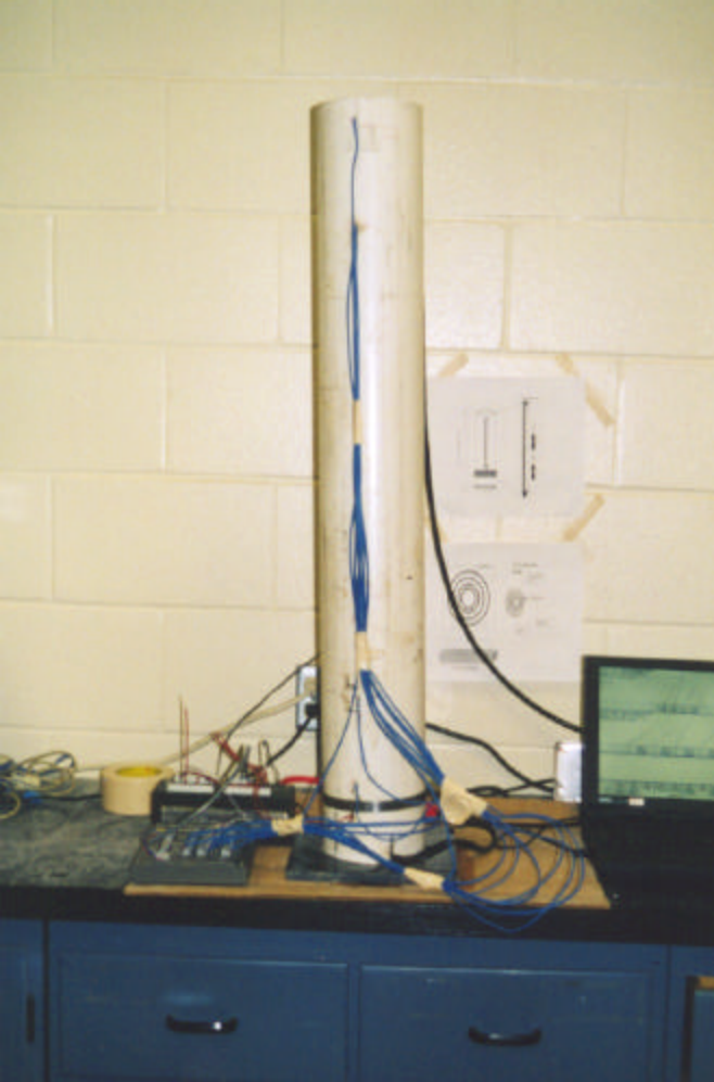
Figure. 1 Soil Column with Multi-Segment TDR probe and thermocouples installed.
