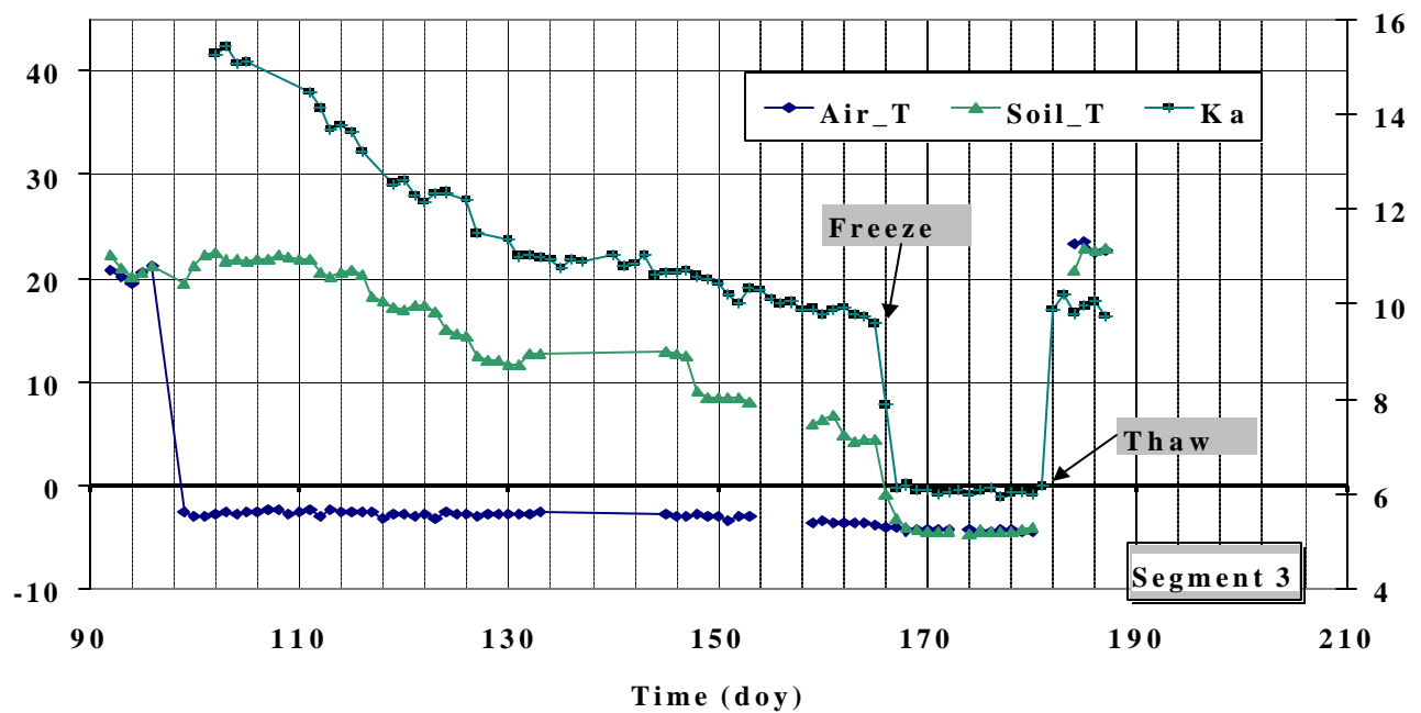
Figure 6 Temperature and Ka vs Time for TDR segment 3 (30-45cm). The Soil_T is the average temperature of the two thermocouples located at the top and bottom of the segment. Segment 3 went through a rapid freeze-thaw cycle on day 165 and day 181 respectively.
