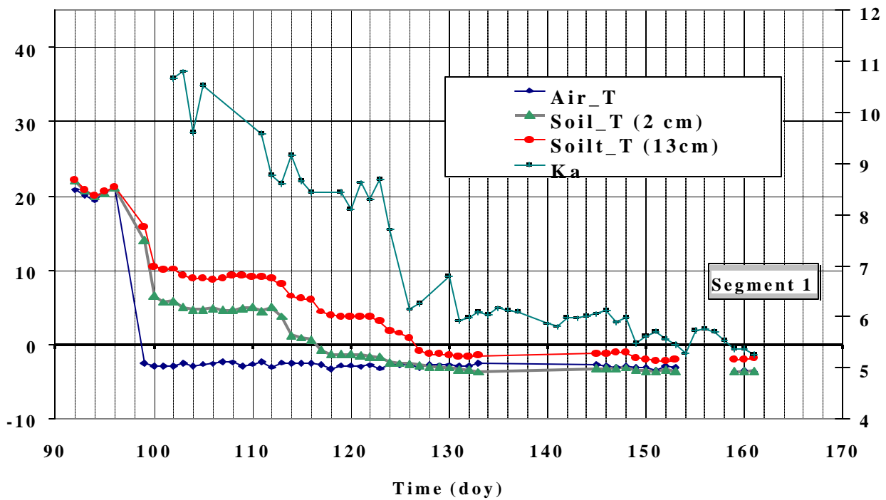
Figure 7 A change in the Ka is evident only after Soil_T (13cm) has dropped below 0 °C. Freezing may be occurring in the upper part of the segment , although it is difficult to detect.
