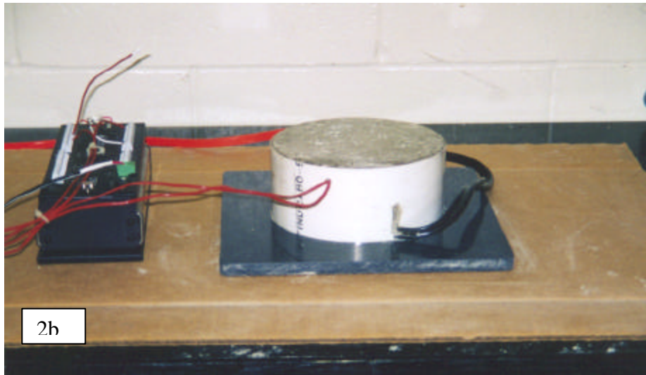
Figure 2 (a) PVC heater core with heating tape and thermocouples. Temperature measurements were taken by a Campbell Scientific Inc. CR10 datalogger. (b) Heater core filled with Quickcrete and CR10 datalogger.
